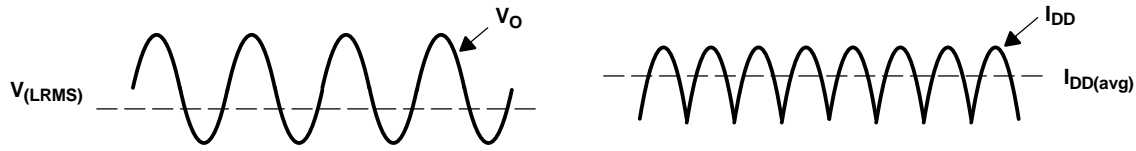
Figure 38. Voltage and Current Waveforms for BTL Amplifiers
