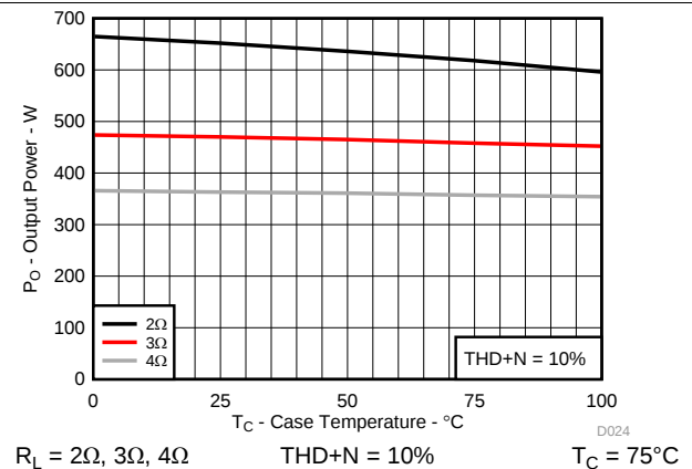
Figure 24. Output Power vs Case Temperature
