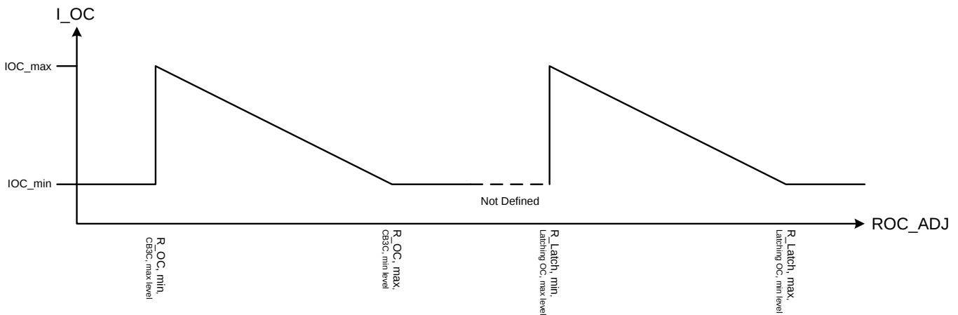
FIG 27. OC Threshold versus OC_ADJ Resistor Value Example
