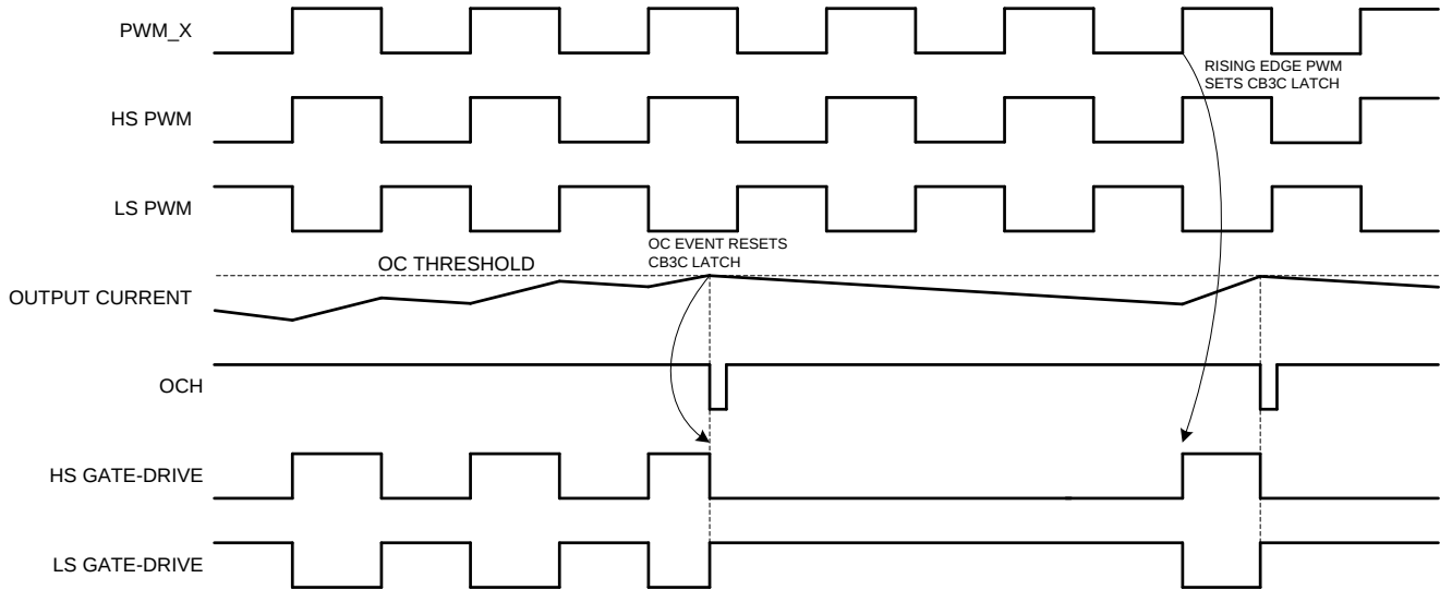
FIG 26. CB3C Timing Example
