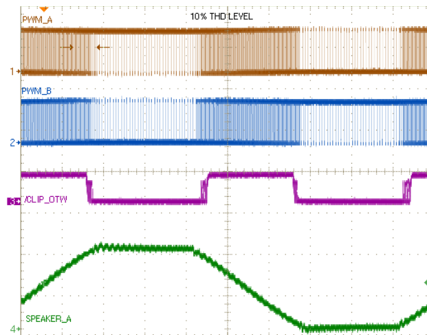
図 28. Signal Clipping PWM and Speaker Output Signals
