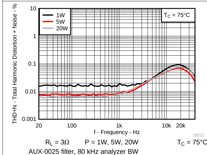
FIG 12. Total Harmonic Distortion+Noise vs Frequency
