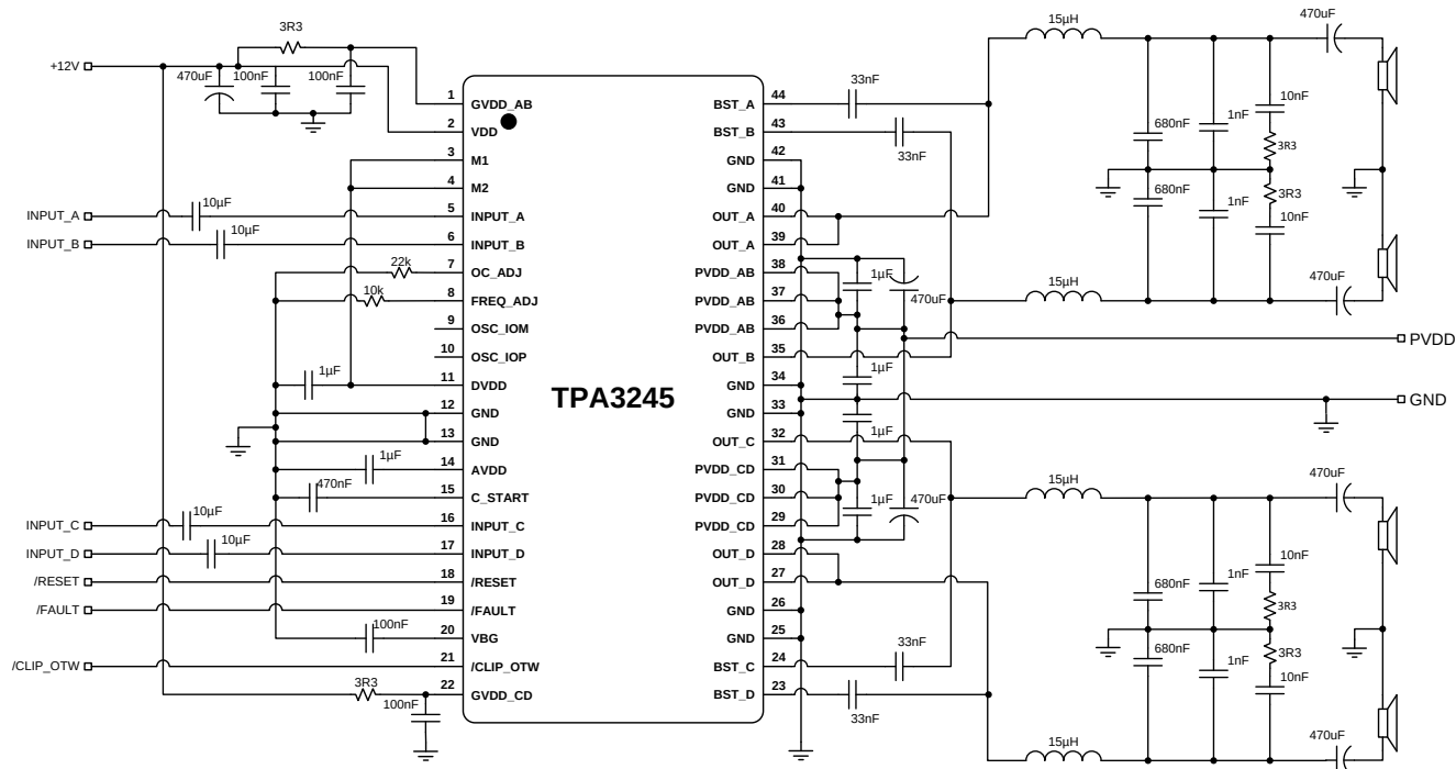
☒ 27. Typical Single Ended (1N) SE Application
