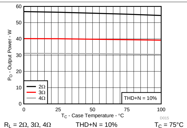
FIG 15. Output Power vs Case Temperature
