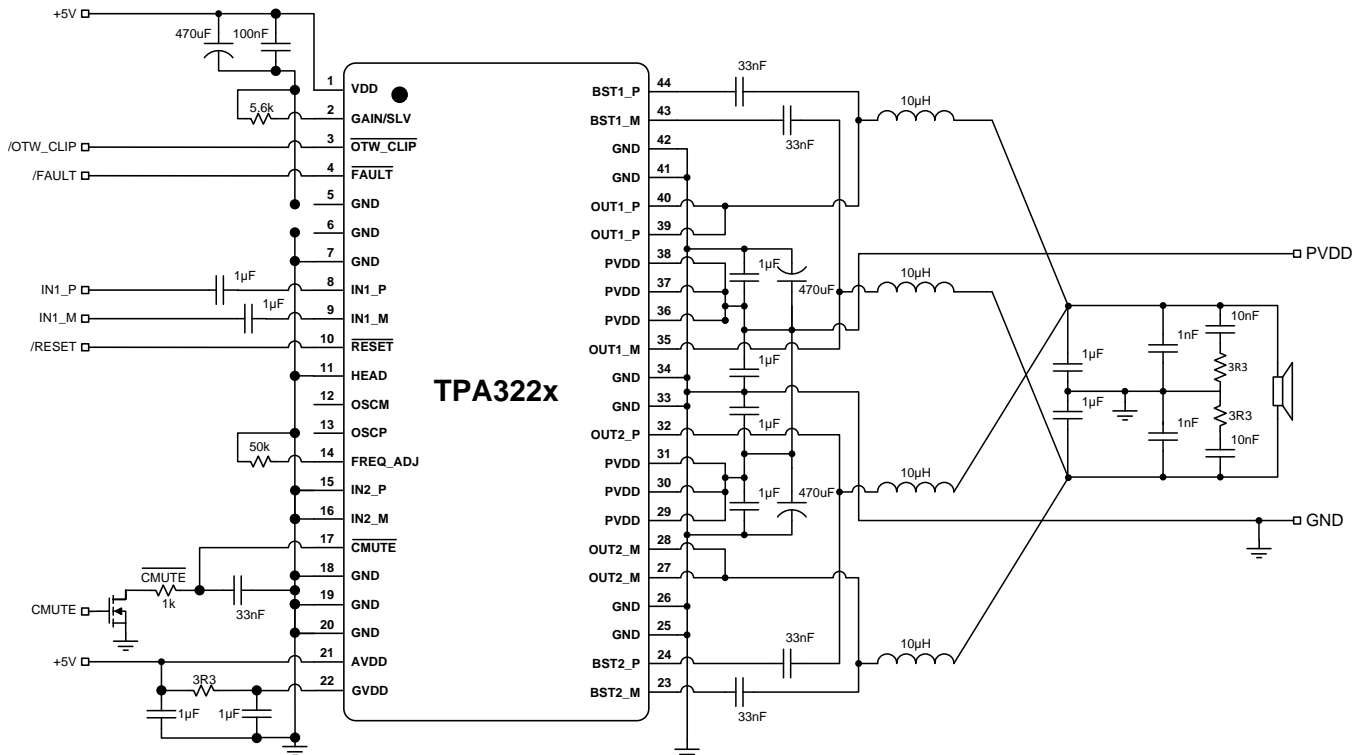
図 52. Typical Differential (2N) AD-Mode PBTL Application
