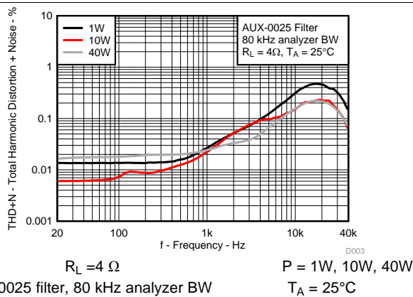
Figure 3. Total Harmonic Distortion+Noise vs Frequency, AD-mode
