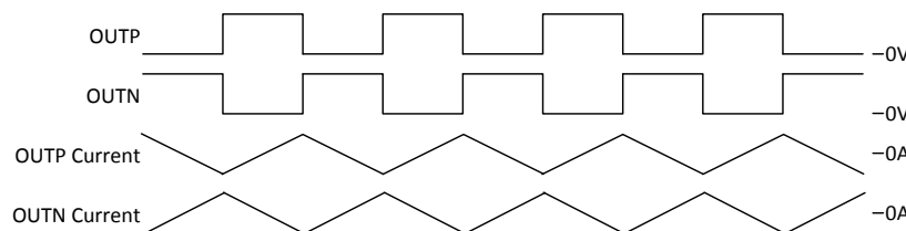
FIG 36. AD Mode Output Waveforms, Idle
