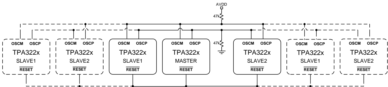
FIG 33. Gain and Master PCB Implementation
