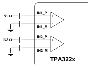
図 31. Single Ended Audio Input Configuration
