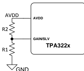
図 32. Gain and Master / Slave Setup
