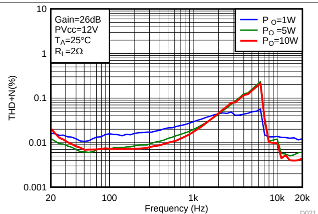
FIG 18. Total Harmonic Distortion + Noise (PBTL) vs Frequency
