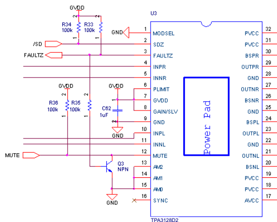
FIG 28. MUTE Driven by Inverted FAULTZ
