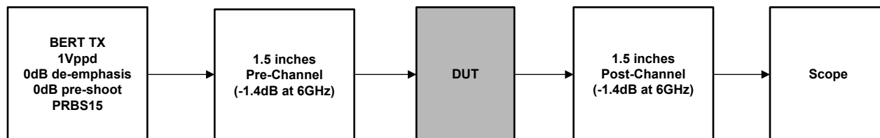
Figure 8-3. Test Setup
