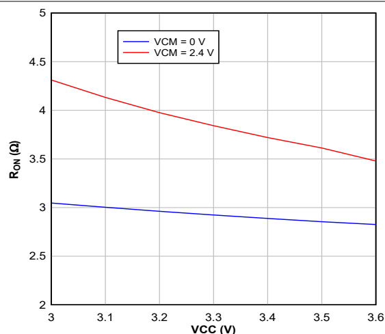
Fig 6-8. R_{ON} vs Supply Voltage VCC
