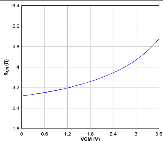
Fig 6-7. R_{ON} vs Common Mode Voltage VCM
