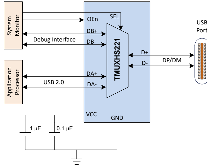
8-1. Routing Debug Signals to USB Port
