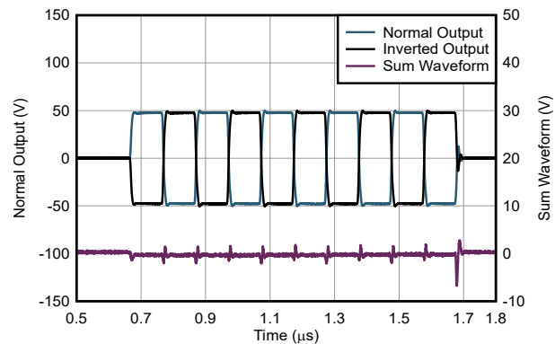
8-11. Pulser + TMUX9616, Mux Output Side, \pm 60V Pulser Supplies, 5MHz, 5 Cycles, 100\Omega \parallel 100pF Load
