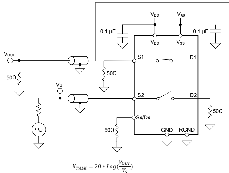
図 6-4. Crosstalk Measurement Setup
