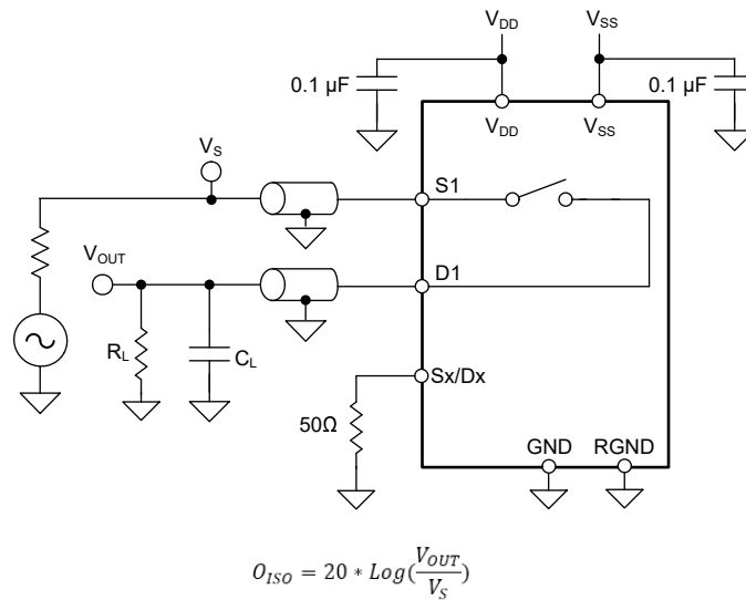
図 6-3. Off Isolation Measurement Setup
