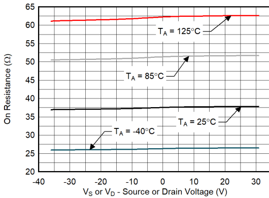
Figure 7-1. On-Resistance vs Source or Drain Voltage
