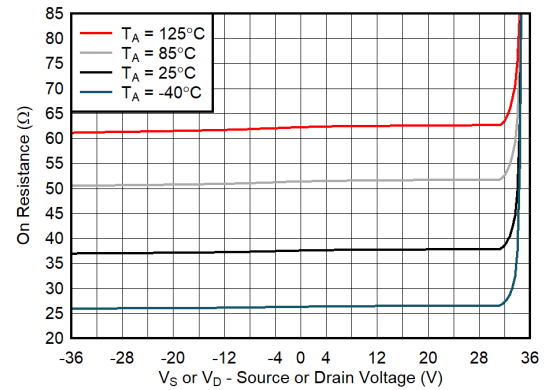
Figure 7-2. On-Resistance vs Source or Drain Voltage
