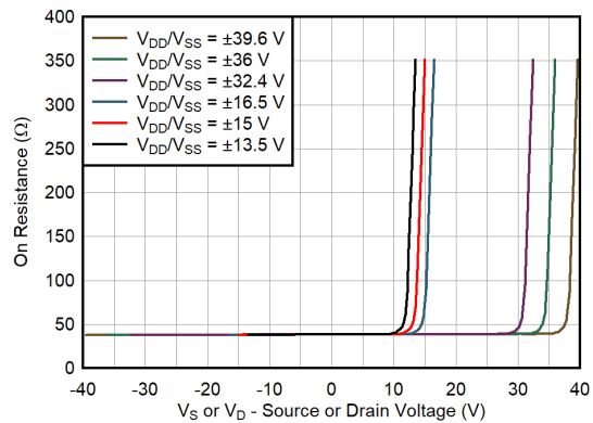
Figure 7-4. On-Resistance vs Source or Drain Voltage
