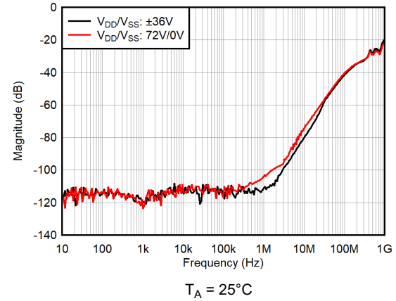
FIG 7-28. Off Isolation vs Frequency
