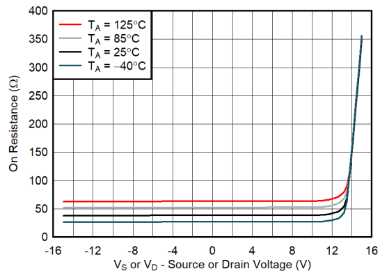
Figure 7-6. On-Resistance vs Source or Drain Voltage
