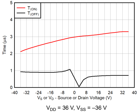
FIG 7-27. Turn-On and Turn-Off Times vs Source Voltage
