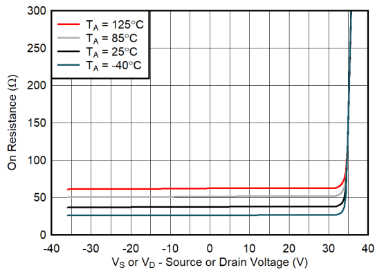
Figure 7-3. On-Resistance vs Source or Drain Voltage
