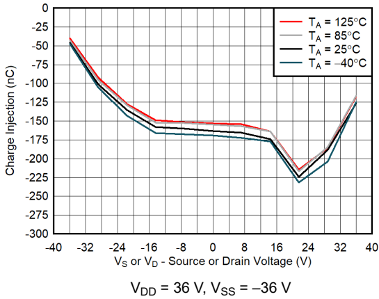
FIG 7-25. Charge Injection vs Source Voltage
