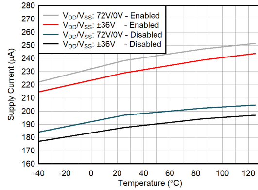
FIG 7-26. Supply Current vs Temperature
