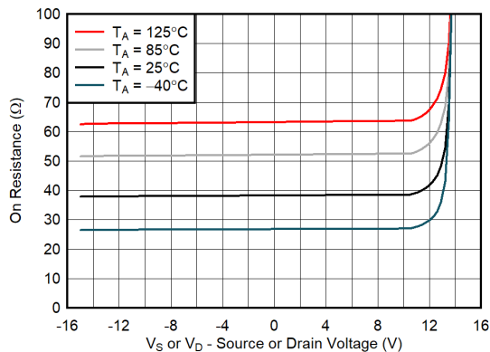
Figure 7-5. On-Resistance vs Source or Drain Voltage
