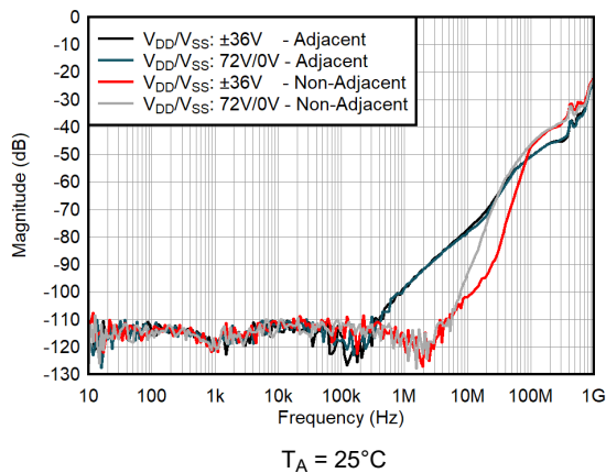
7-29. Crosstalk vs Frequency
