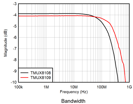
7-30. Insertion Loss vs Frequency
