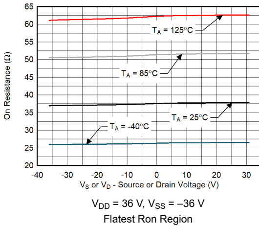
Figure 7-1. On-Resistance vs Source or Drain Voltage
