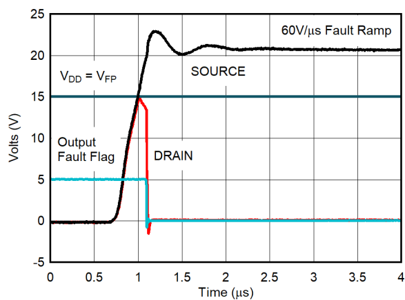
6-25. Drain Output Response - Positive Overvoltage
