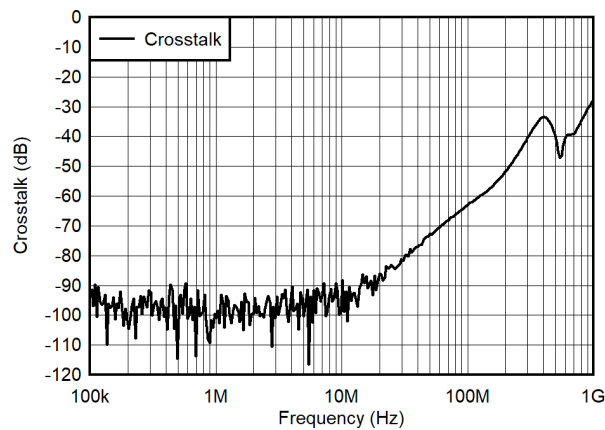
FIG 6-21. Crosstalk vs Frequency
