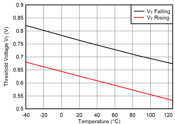
FIG 6-24. Threshold Voltage vs Temperature
