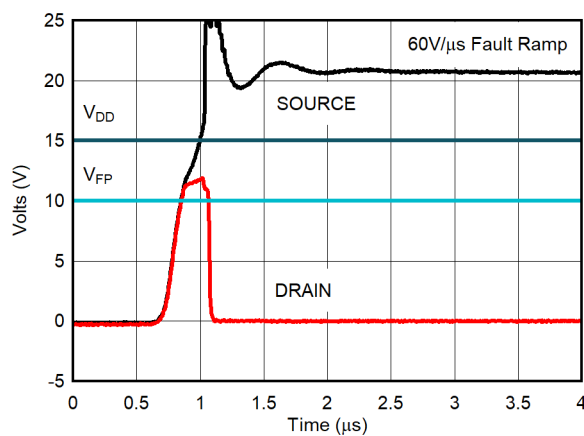
6-26. Drain Output Response - Positive Overvoltage
