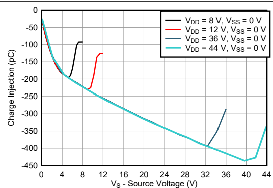
FIG 6-24. Charge Injection vs Source Voltage – Single Supply
