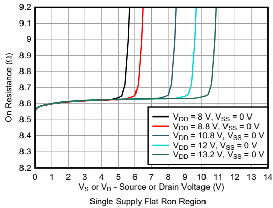
FIG 6-7. On-Resistance vs Source or Drain Voltage
