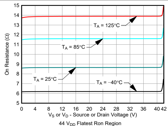
FIG 6-10. On-Resistance vs Source or Drain Voltage
