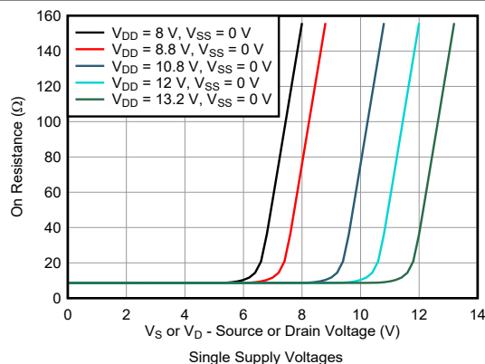
FIG 6-4. On-Resistance vs Source or Drain Voltage
