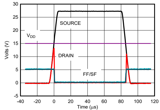
FIG 6-32. Fault Response and Recovery
