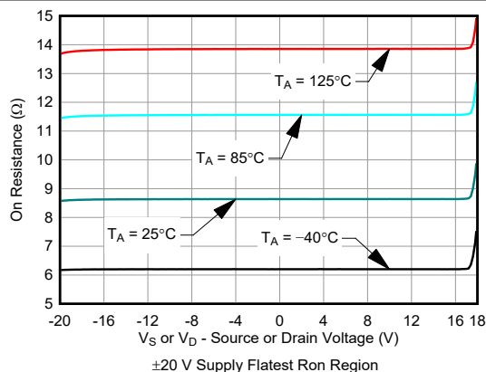
FIG 6-5. On-Resistance vs Source or Drain Voltage
