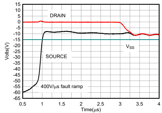
FIG 6-36. Drain Output Recovery – Negative Overvoltage
