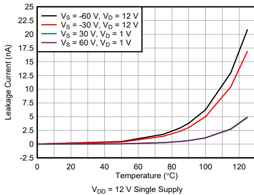
FIG 6-19. I_{D(FA)} Overvoltage Leakage Current vs Temperature
