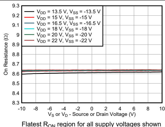
FIG 6-3. On-Resistance vs Source or Drain Voltage
