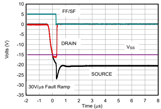
FIG 6-32. Fault Response and Recovery
