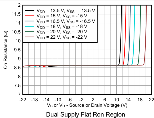
FIG 6-2. On-Resistance vs Source or Drain Voltage
