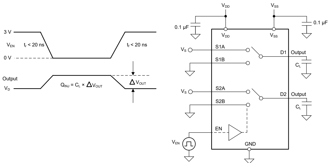
7-13. Charge-Injection Measurement Setup
