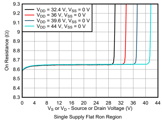
FIG 6-8. On-Resistance vs Source or Drain Voltage
