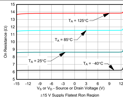
FIG 6-2. On-Resistance vs Source or Drain Voltage
