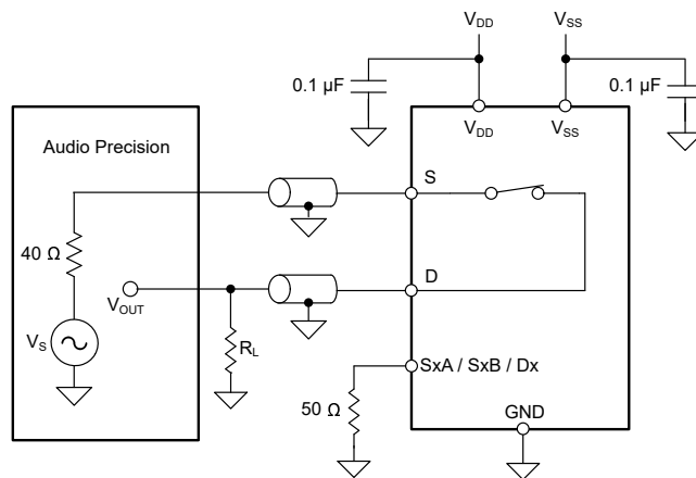
Figure 7-18. THD+N Measurement Setup
