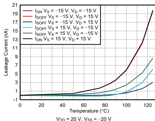
6-14. Leakage Current vs Temperature
