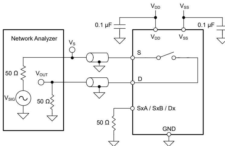
7-14. Off Isolation Measurement Setup
