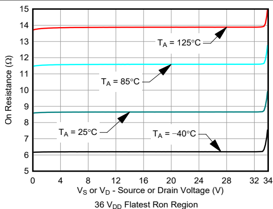
FIG 6-9. On-Resistance vs Source or Drain Voltage
