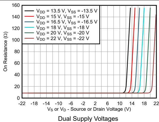
FIG 6-1. On-Resistance vs Source or Drain Voltage
