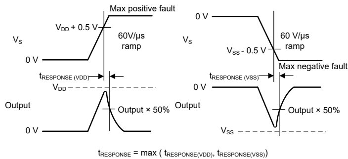
7-9. Fault Response Time Measurement Setup
