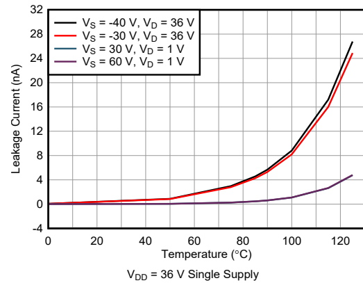
FIG 6-20. I_{D(FA)} Overvoltage Leakage Current vs Temperature
