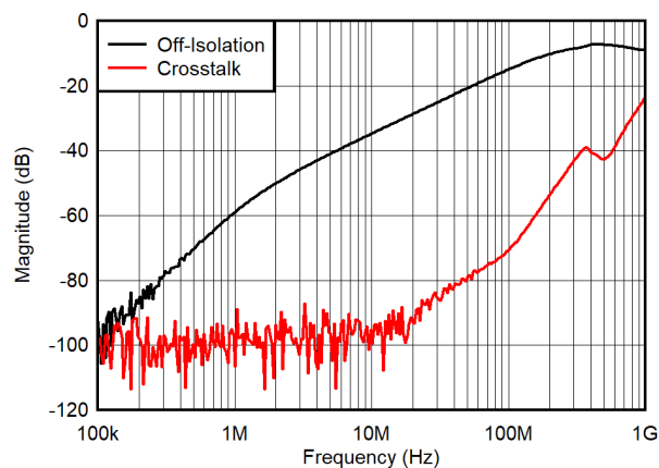
7-29. Crosstalk and Off Isolation vs Frequency
