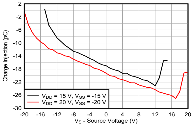
FIG 7-25. Charge Injection vs Source Voltage – Dual Supply
