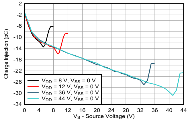
FIG 7-26. Charge Injection vs Source Voltage – Single Supply
