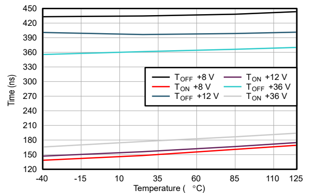
FIG 7-28. Transition Times vs Temperature
