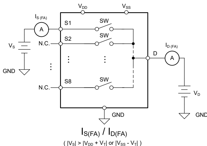
8-4. Measurement Setup for Input and Output Leakage Current under Overvoltage Fault with Normal Supplies
