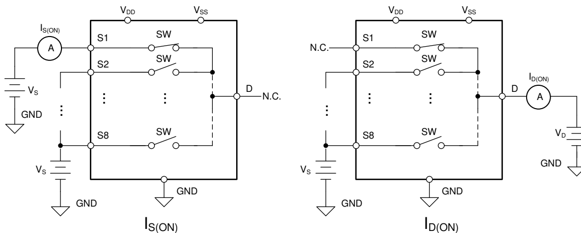
8-3. On-Leakage Measurement Setup
