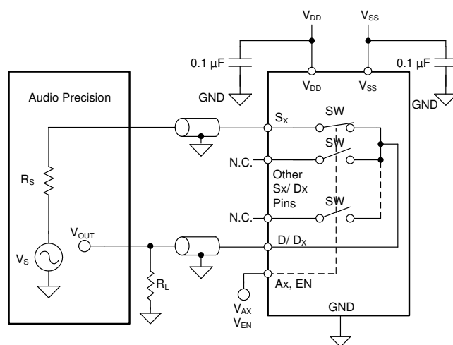
8-16. THD+N Measurement Setup
