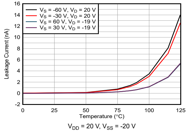
7-20. I_{D(FA)} Overvoltage Leakage Current vs Temperature
