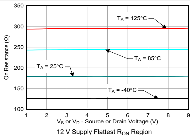
FIG 7-8. On-Resistance vs Source or Drain Voltage
