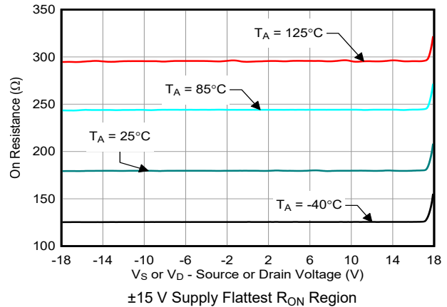
7-4. On-Resistance vs Source or Drain Voltage
