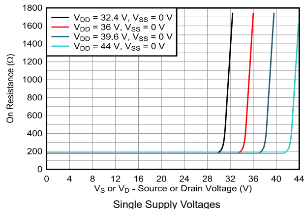
FIG 7-9. On-Resistance vs Source or Drain Voltage
