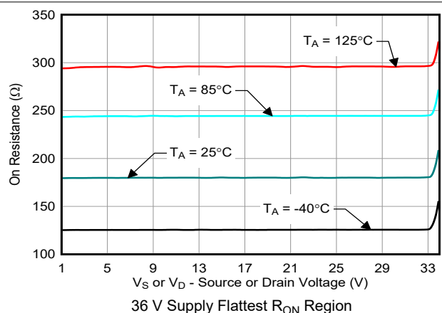
FIG 7-11. On-Resistance vs Source or Drain Voltage
