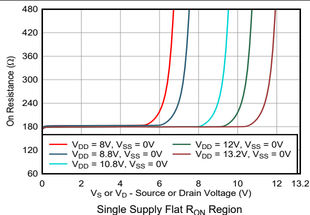
FIG 7-7. On-Resistance vs Source or Drain Voltage
