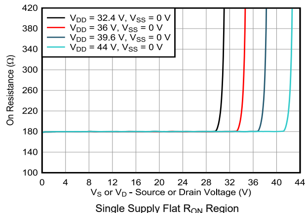
FIG 7-10. On-Resistance vs Source or Drain Voltage
