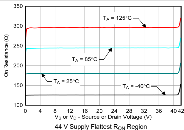
FIG 7-12. On-Resistance vs Source or Drain Voltage
