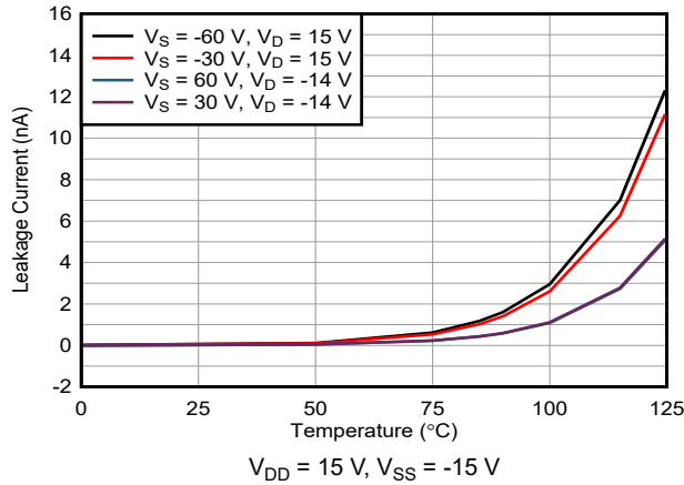
7-19. I_{D(FA)} Overvoltage Leakage Current vs Temperature
