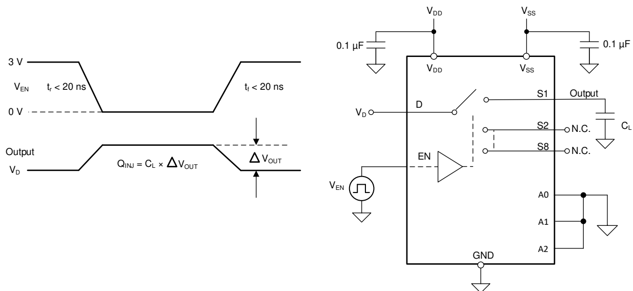
図 7-9. Charge-Injection Measurement Setup
