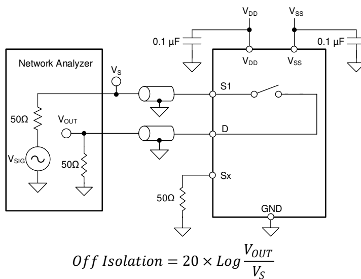
図 7-10. Off Isolation Measurement Setup
