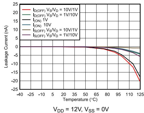
図 6-12. Leakage Current vs Temperature
