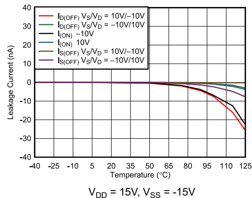
図 6-10. Leakage Current vs Temperature
