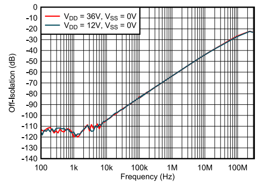
Figure 6-23. Off-Isolation vs Frequency
