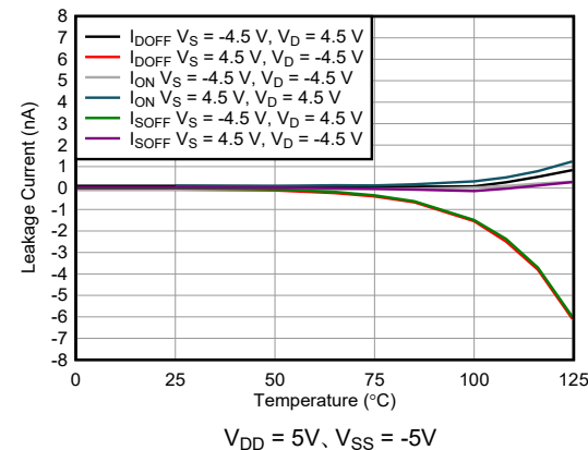
図 5-10. Leakage Current vs Temperature
