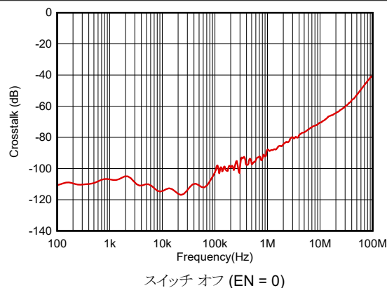
図 5-22. Crosstalk vs Frequency
