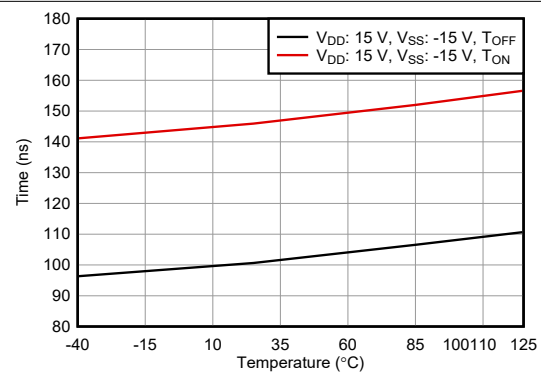
5-18. T_{ON} and T_{OFF} vs Temperature
