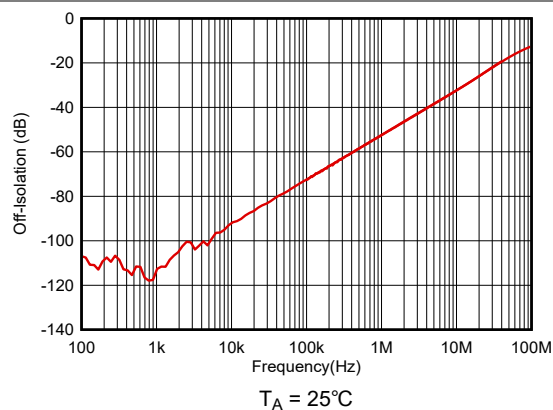
図 5-20. Off-Isolation vs Frequency
