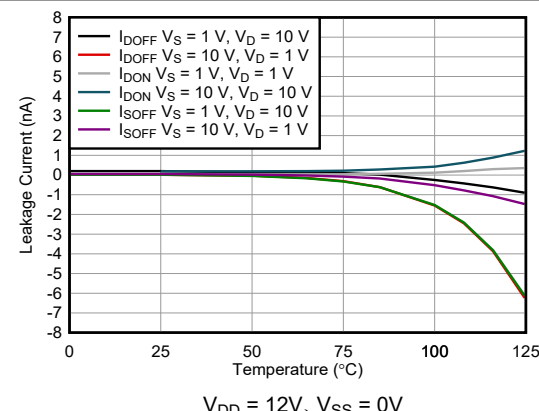
図 5-12. Leakage Current vs Temperature
