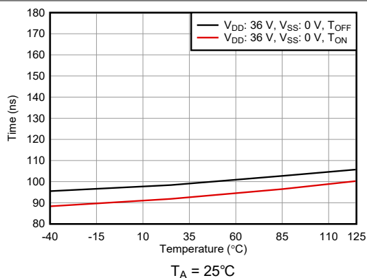
図 5-19. T_{ON} and T_{OFF} vs Temperature
