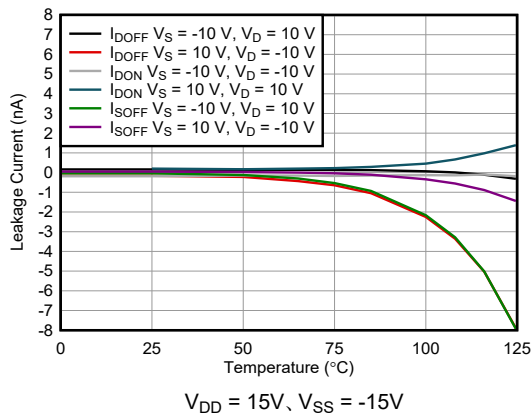
図 5-9. Leakage Current vs Temperature
