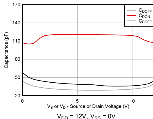
図 5-28. Capacitance vs Source Voltage or Drain Voltage
