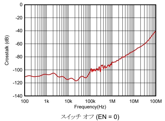
図 5-22. Crosstalk vs Frequency
