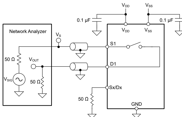
図 6-8. Off Isolation Measurement Setup
