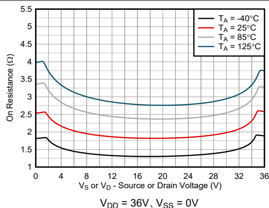
図 5-8. On-Resistance vs Temperature
