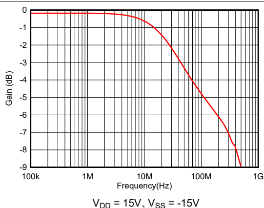
図 5-25. On Response vs Frequency
