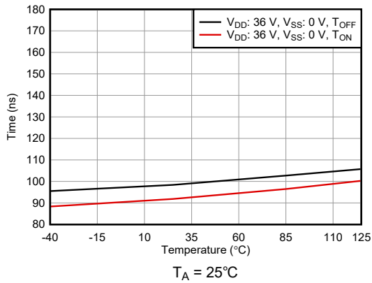
図 5-19. T_{ON} and T_{OFF} vs Temperature
