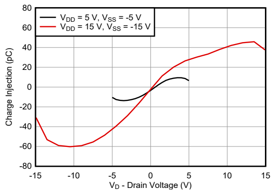
5-15. Charge Injection vs Drain Voltage – Dual Supplies
