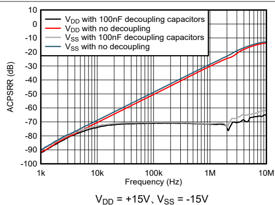
図 5-26. ACPSRR vs Frequency
