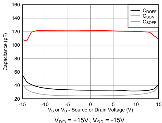
図 5-27. Capacitance vs Source Voltage or Drain Voltage
