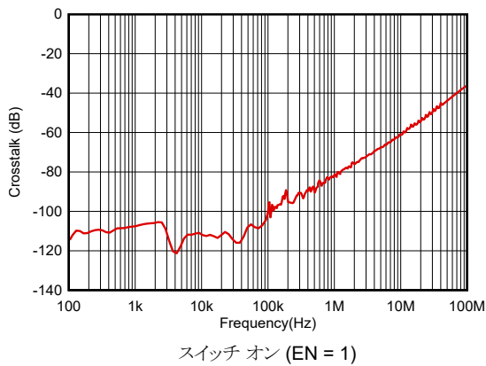
図 5-21. Crosstalk vs Frequency
