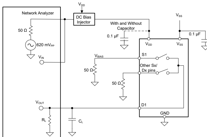
FIG 6-12. AC PSRR Measurement Setup
