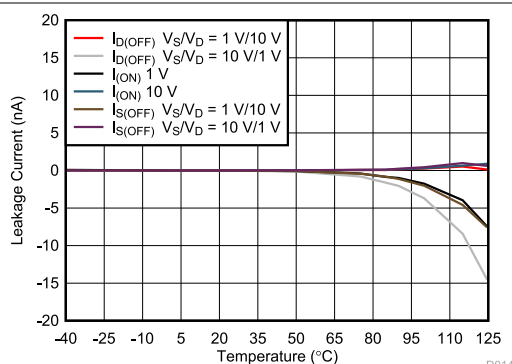
図 5-13. Leakage Current vs Temperature
