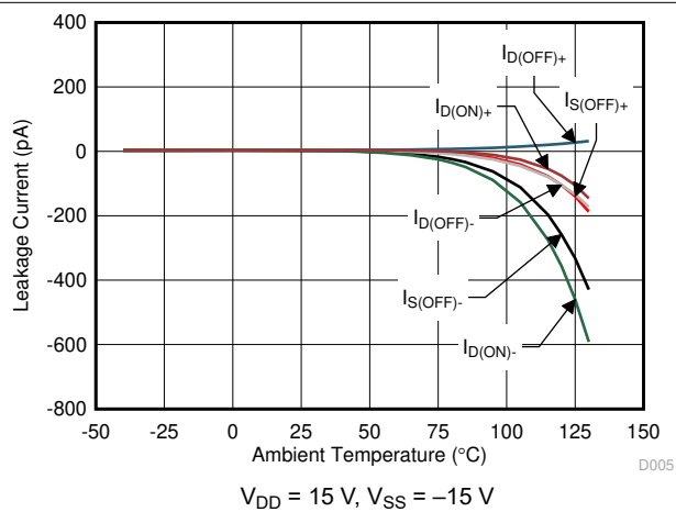
FIG 6-5. Leakage Current vs Temperature
