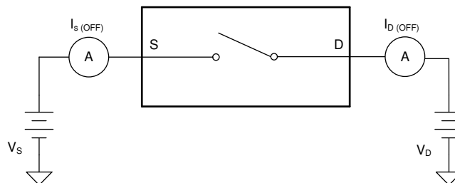
図 8-2. Off-Leakage Measurement Setup
