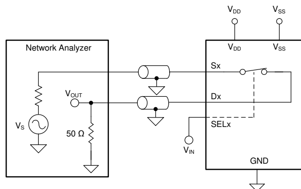
8-9. Bandwidth Measurement Setup
