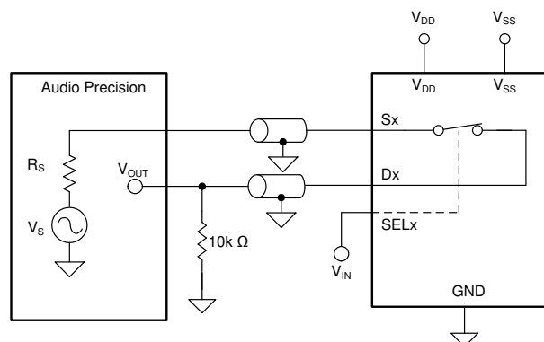
8-10. THD+N Measurement Setup
