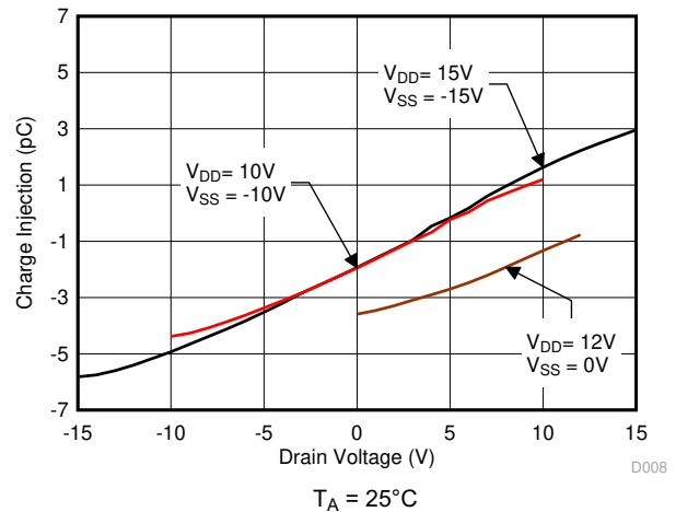
FIG 6-8. Charge Injection vs Drain Voltage
