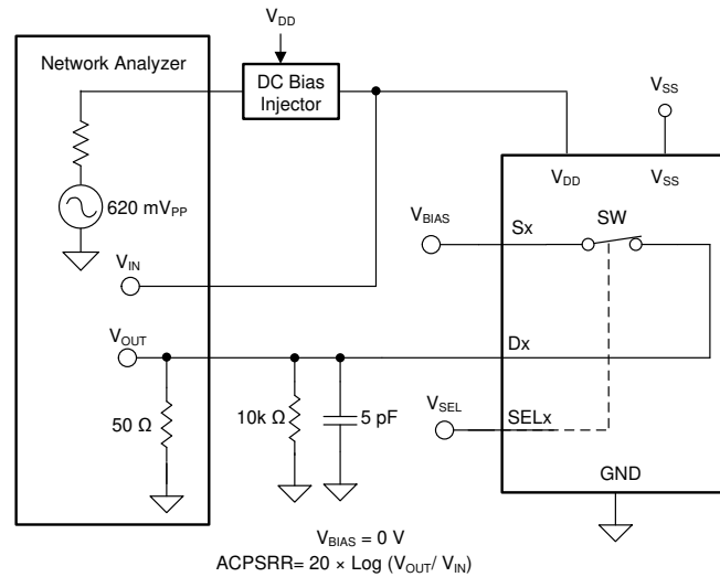
8-11. AC PSRR Measurement Setup
