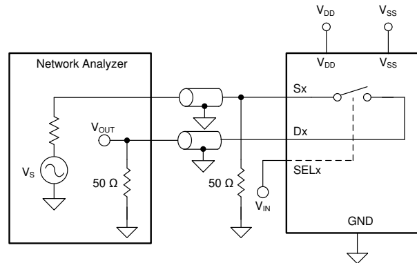
8-7. Off Isolation Measurement Setup
