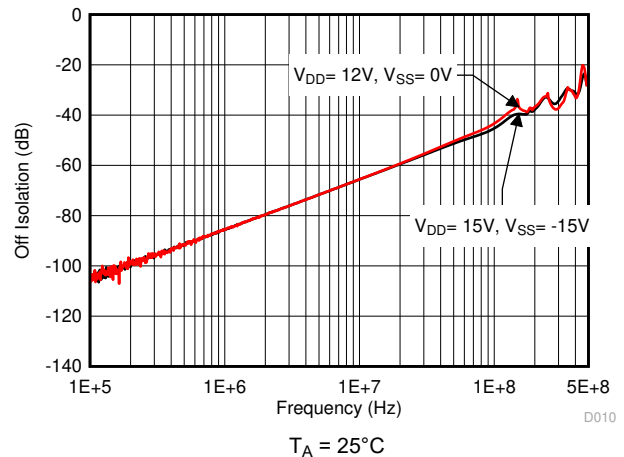
FIG 6-10. Off Isolation vs Frequency
