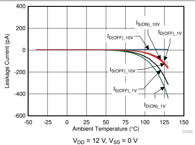
FIG 6-6. Leakage Current vs Temperature
