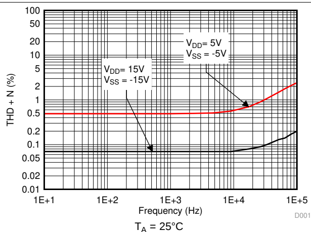
图 12. THD+N vs Frequency
