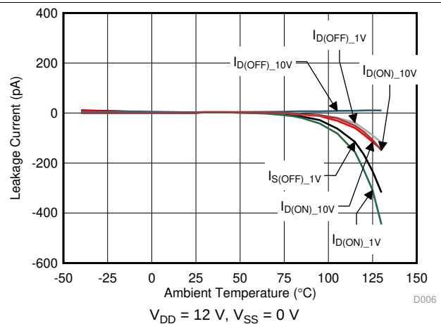
FIG 6. Leakage Current vs Temperature
