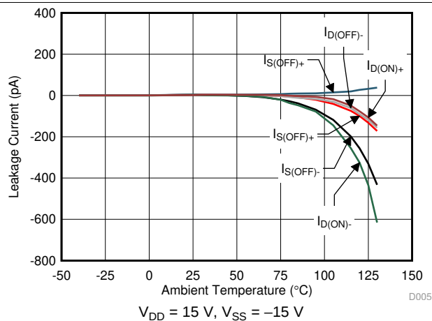
FIG 5. Leakage Current vs Temperature
