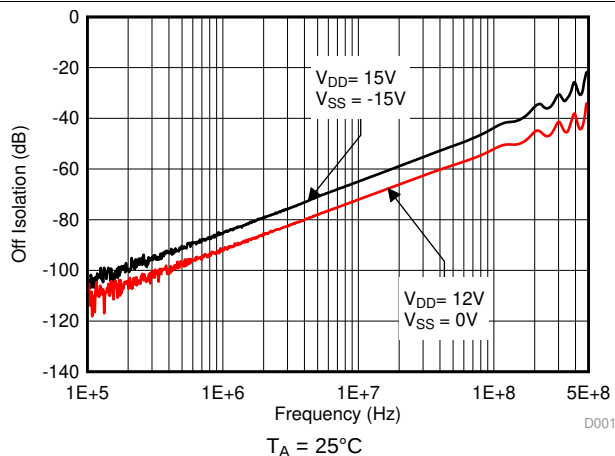
图 10. Off Isolation vs Frequency
