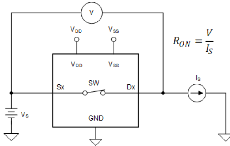
6-1. On-Resistance Measurement Setup
