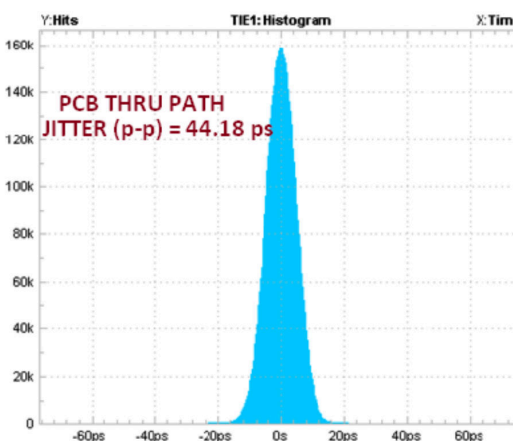
Figure 9-15. Time Interval Error Histogram: 4.5 Gbps with No Device
