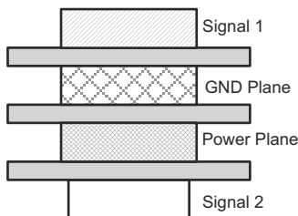
Figure 9-18. Four-Layer Board Stack-Up
