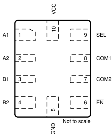
図 5-1. RSE Package, 10-Pin UQFN (Top View)
