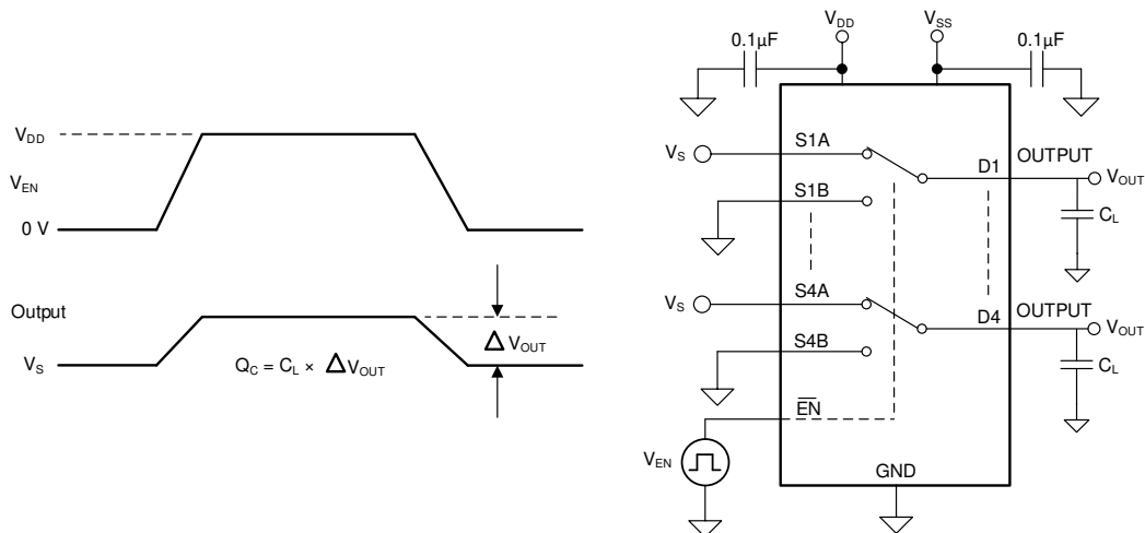
図 7-7. Charge-Injection Measurement Setup
