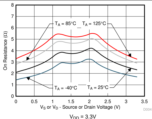
図 6-4. On-Resistance vs Temperature
