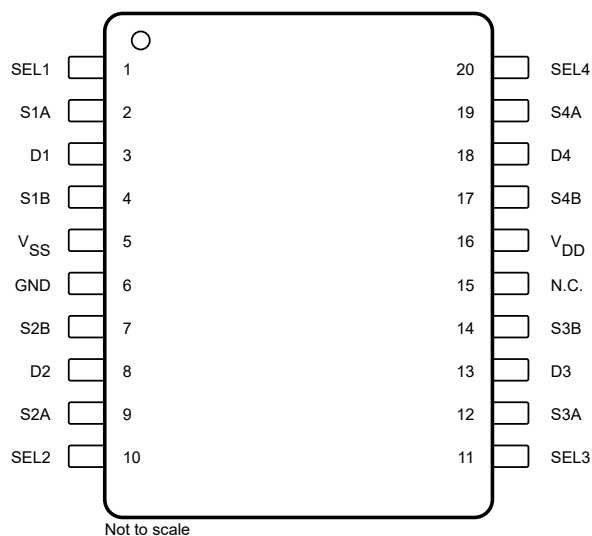
図 5-2. TMUX1134: PW Package, 20-Pin TSSOP (Top View)
