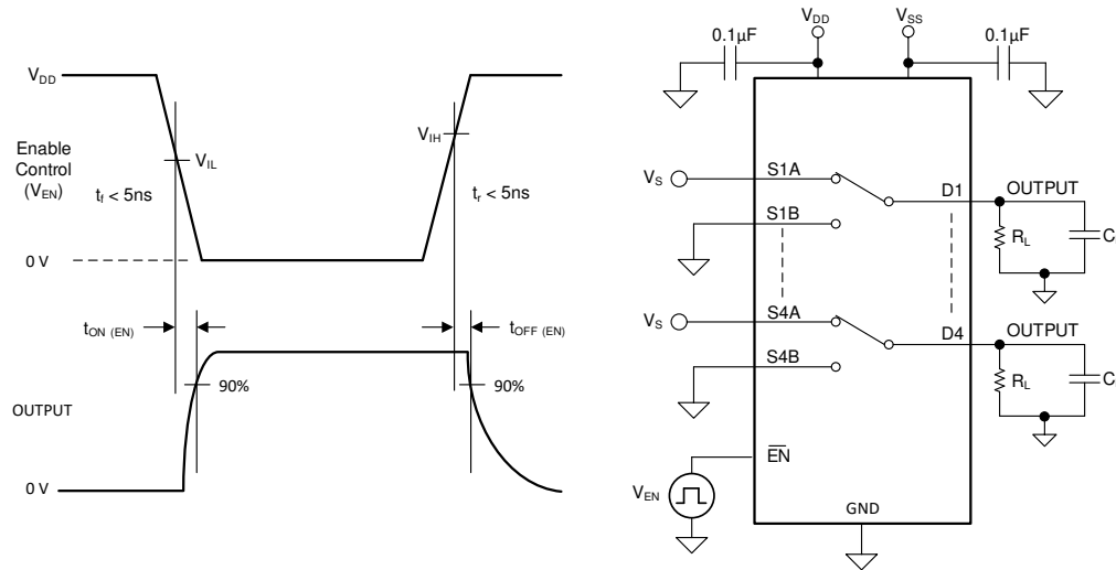
図 7-6. Turn-On and Turn-Off Time Measurement Setup
