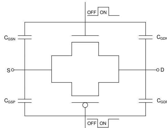
Figure 7-13. Transmission Gate Topology
