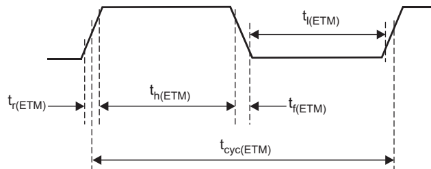
Figure 6-24. ETMTRACECLKOUT Timing
