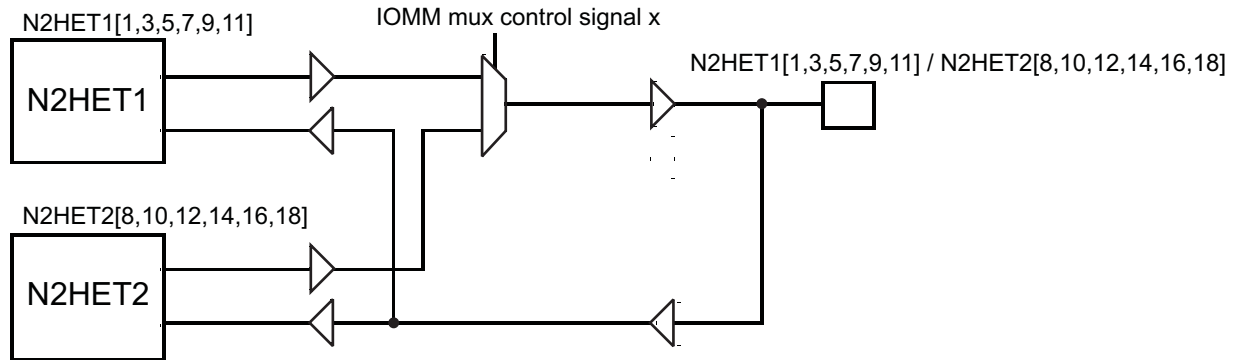
Figure 7-7. N2HET Monitoring
