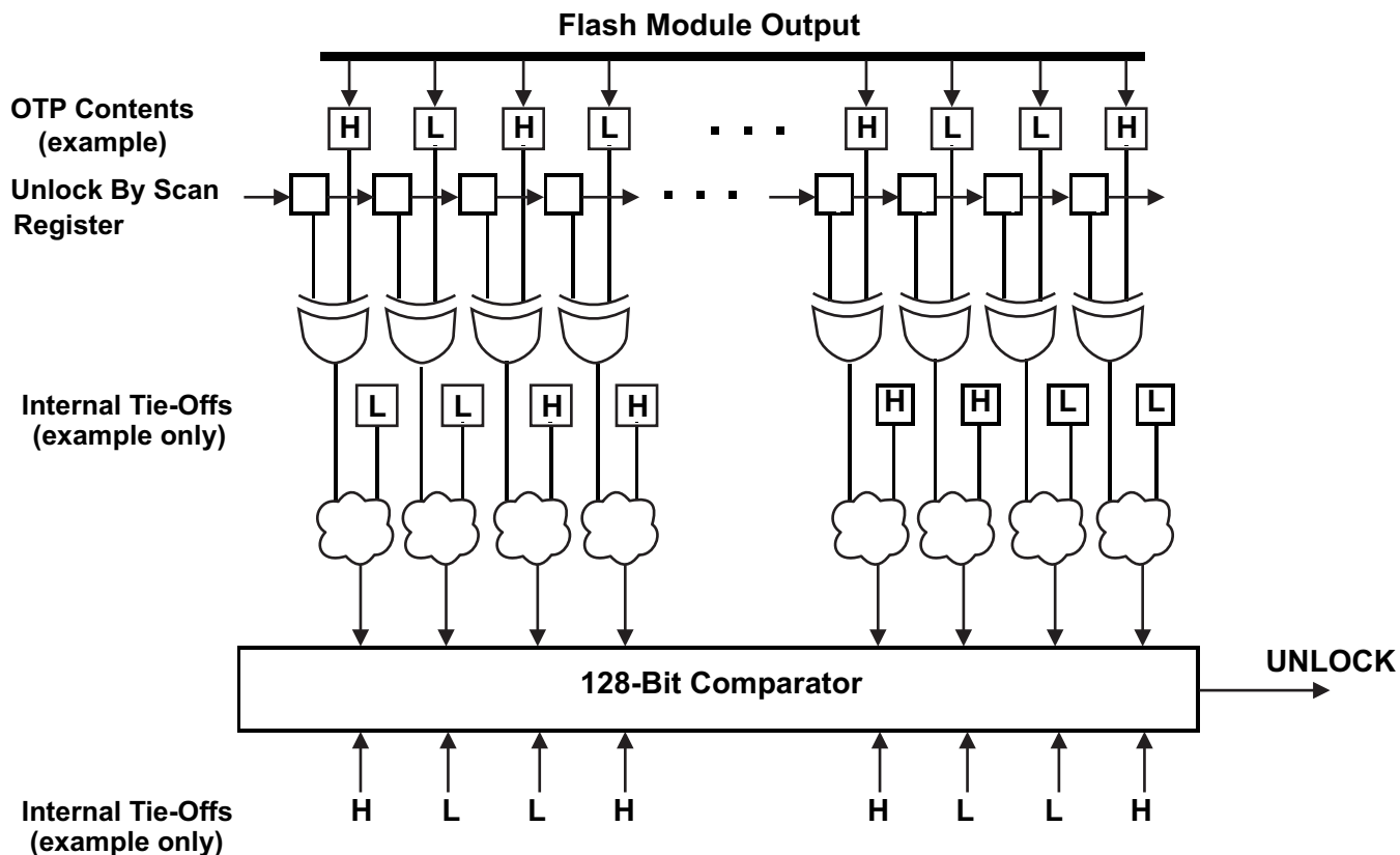
FIG 5-16. AJSM Unlock
