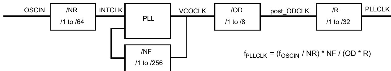
☒ 5-6. PLL Block Diagram
