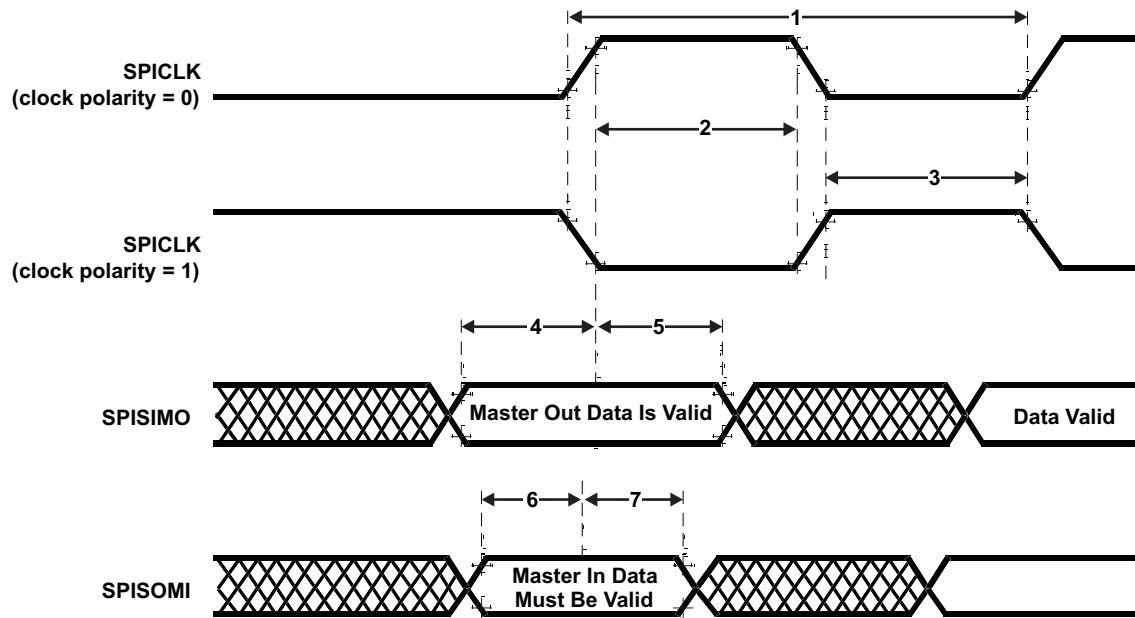
図 6-22. SPI Master Mode External Timing (CLOCK PHASE = 1)
