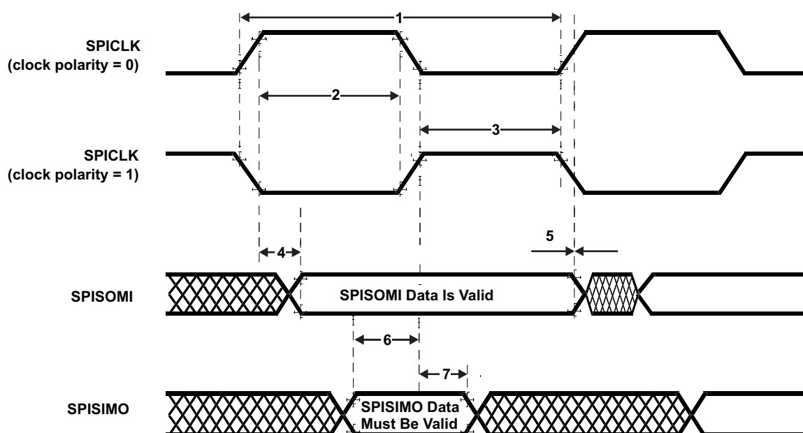
❑ 6-24. SPI Slave Mode External Timing (CLOCK PHASE = 0)
