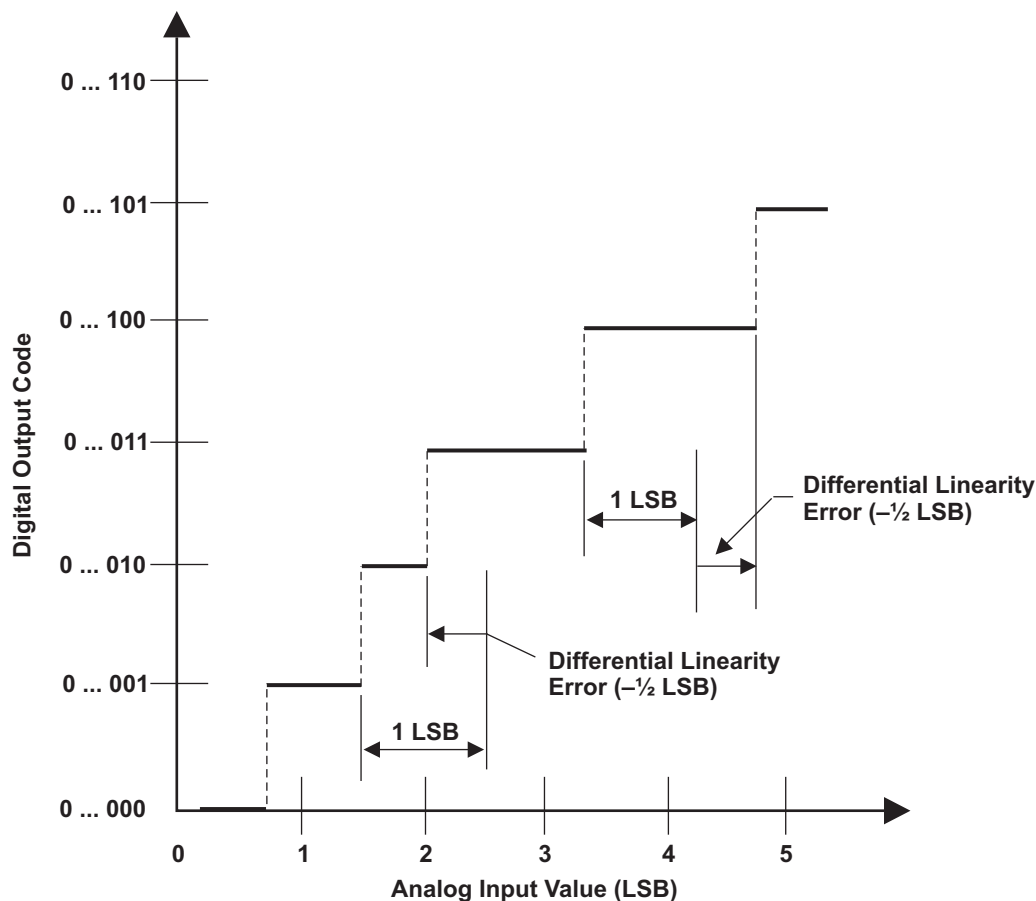
Figure 6-13. Differential Nonlinearity (DNL) Error (A)
