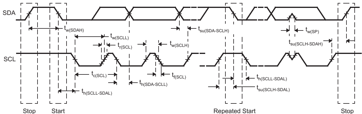
Figure 7-19. I2C Timings
