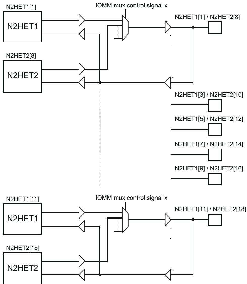
8-17. N2HET Monitoring
