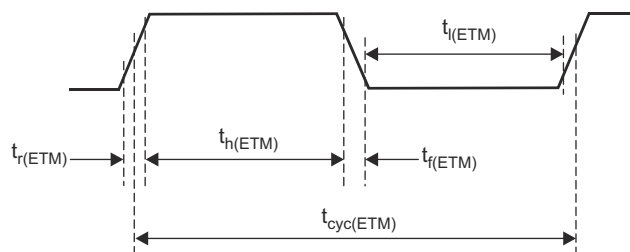
図 7-30. ETMTRACECLKOUT Timing
