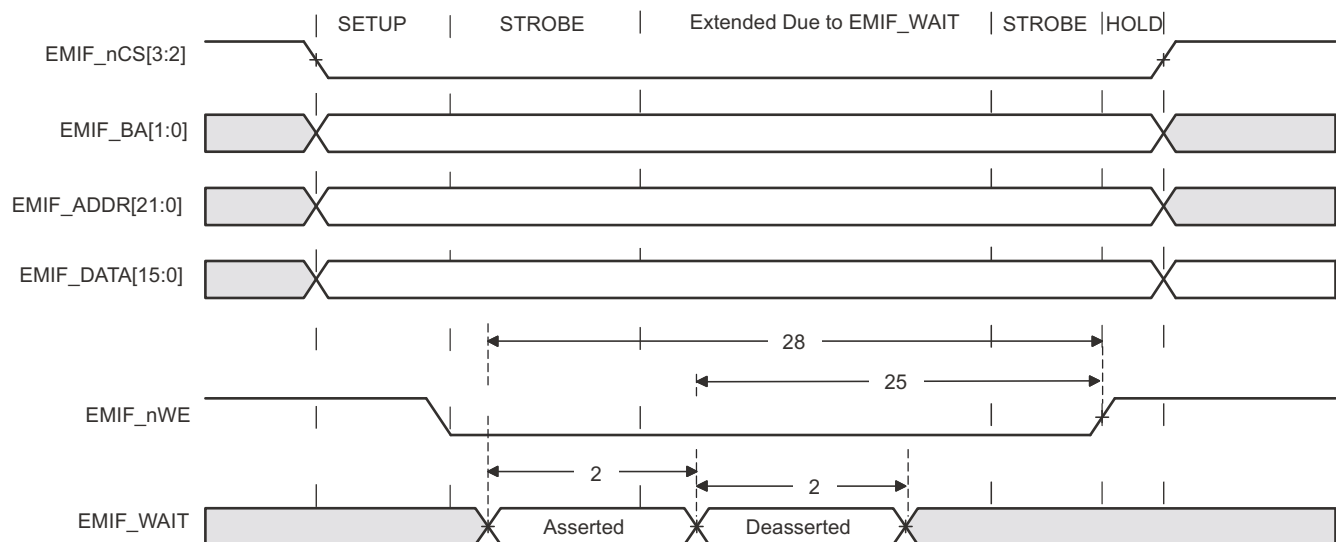
図 7-14. EMIFnWAIT Write Timing Requirements
