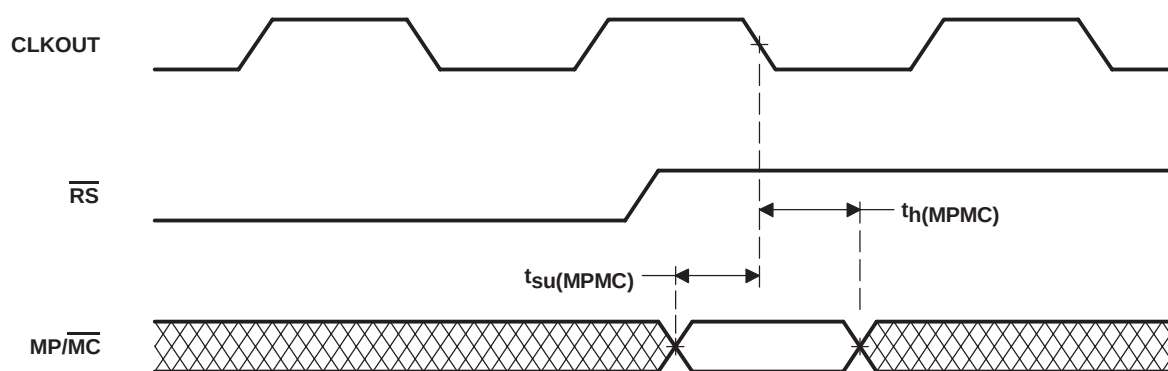
Figure 5-16. MP/MC Timing
