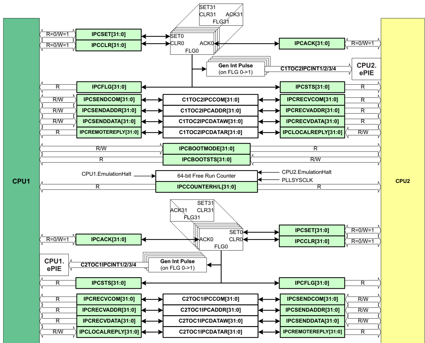
✎ 5-4. IPC Architecture
