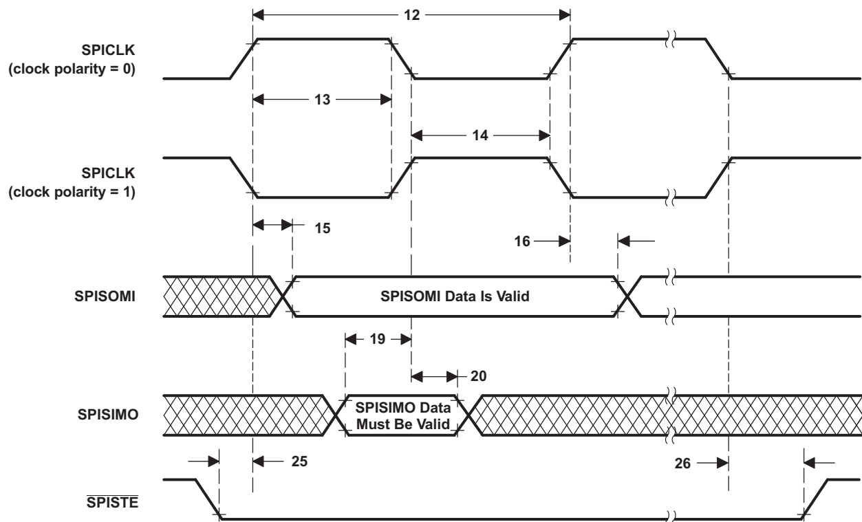
4-75. High-Speed SPI Slave Mode External Timing (Clock Phase = 0)
