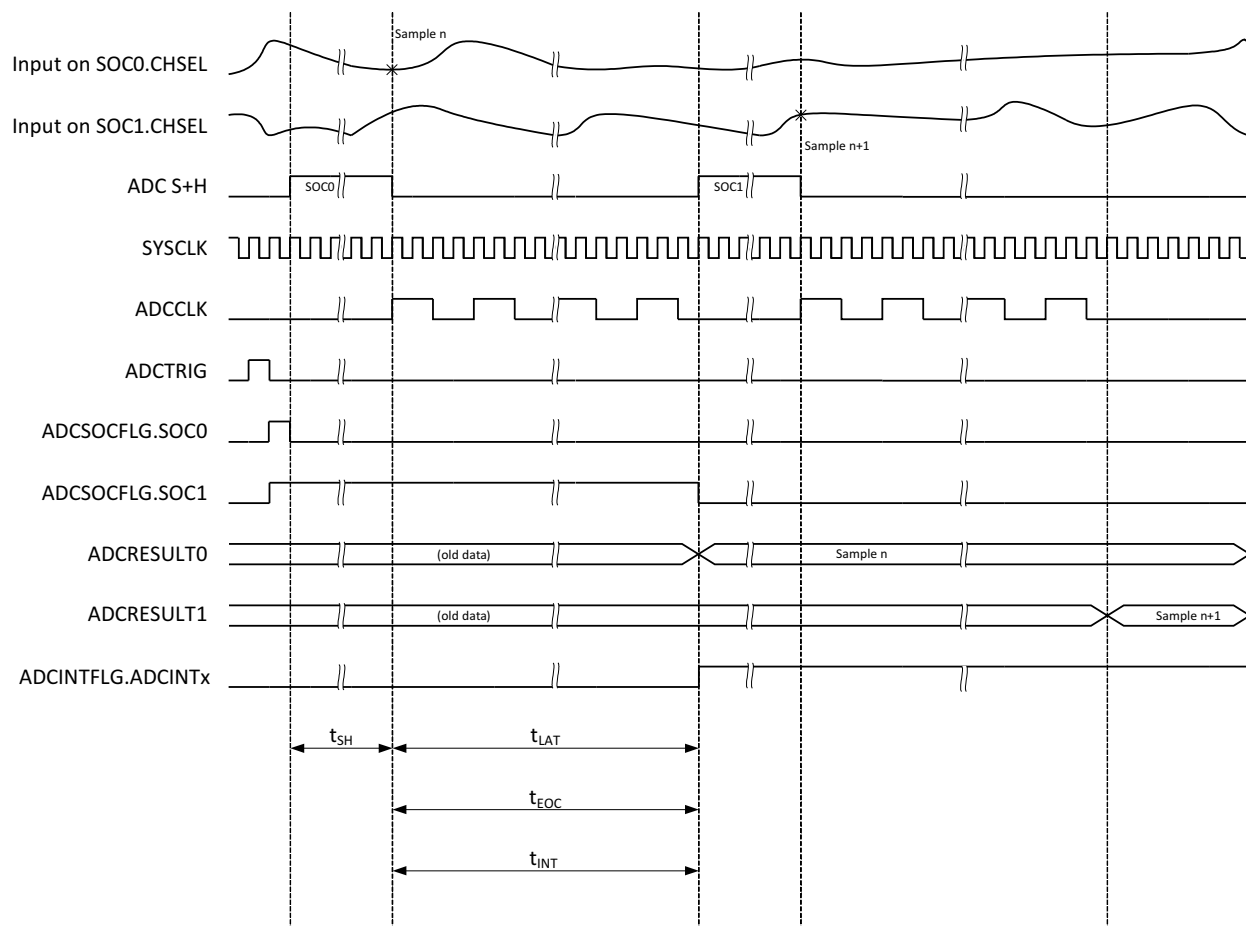
❏ 4-35. ADC Timings for 16-Bit Mode
