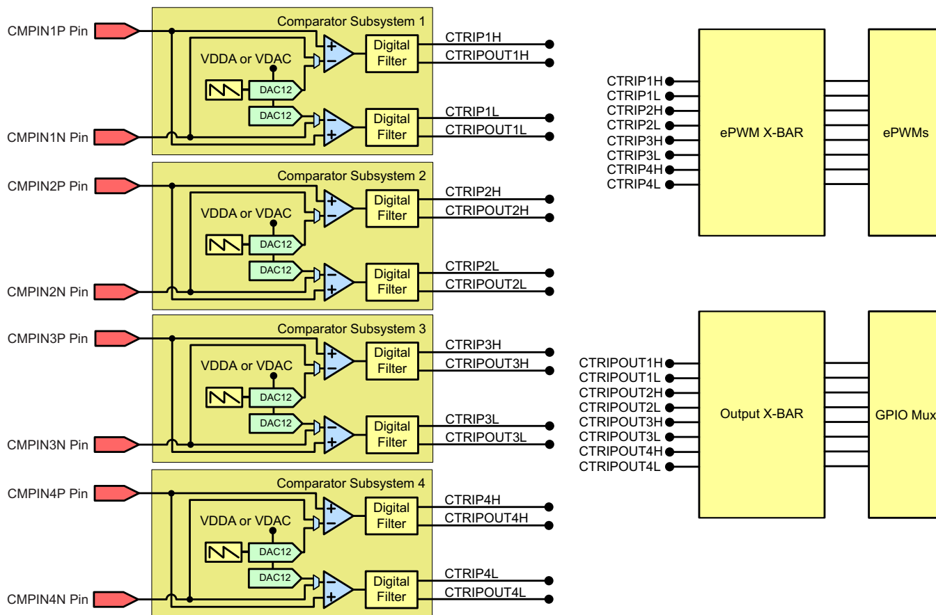
图 4-37. CMPSS Connectivity (100-Pin PZP)
