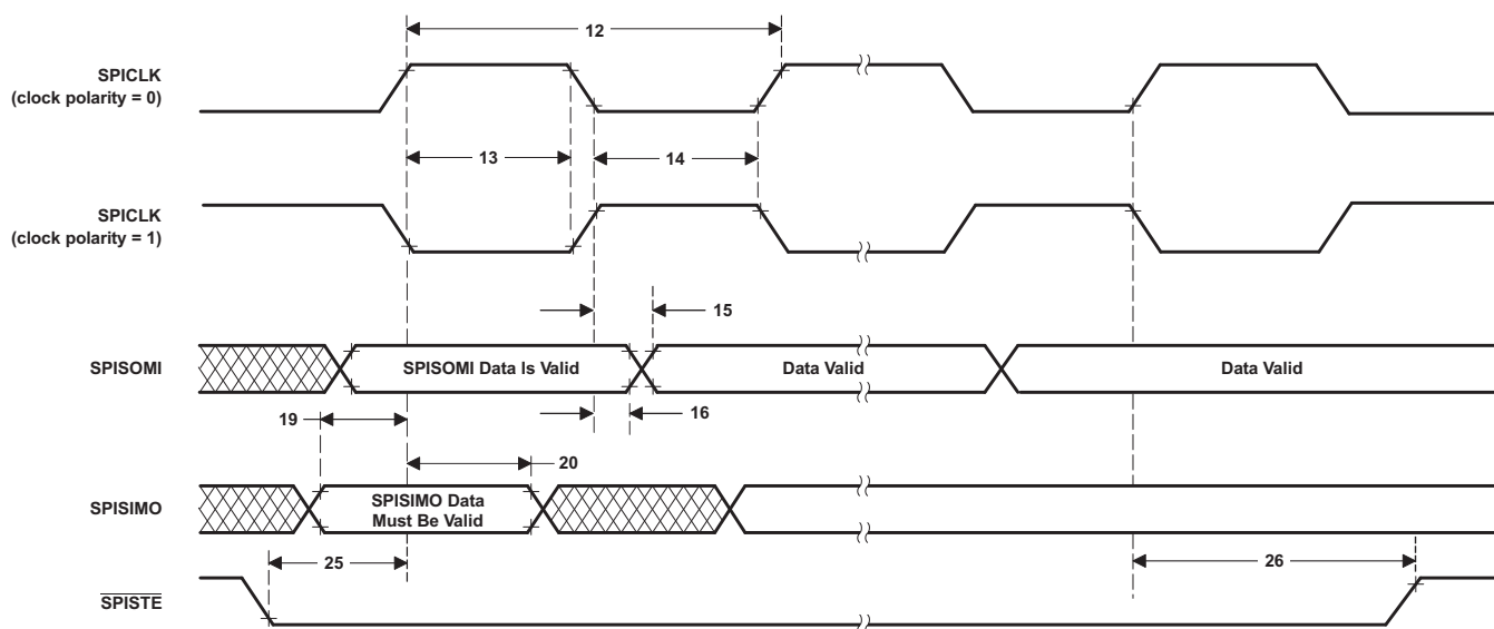
图 4-76. High-Speed SPI Slave Mode External Timing (Clock Phase = 1)
