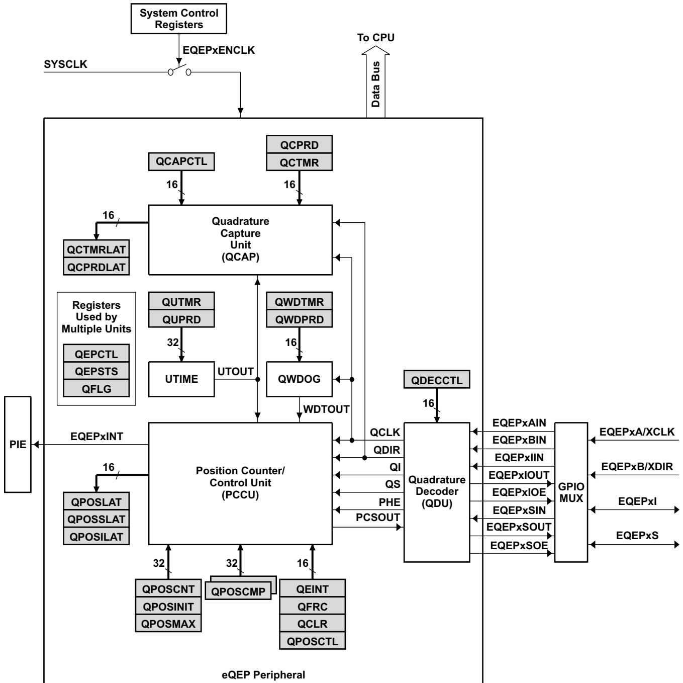
4-53. eQEP Block Diagram
