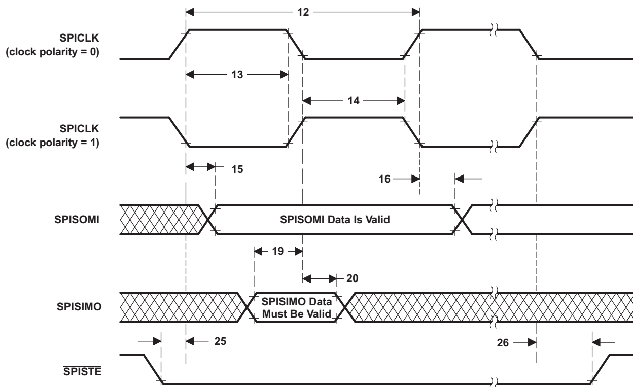
4-71. SPI Slave Mode External Timing (Clock Phase = 0)
