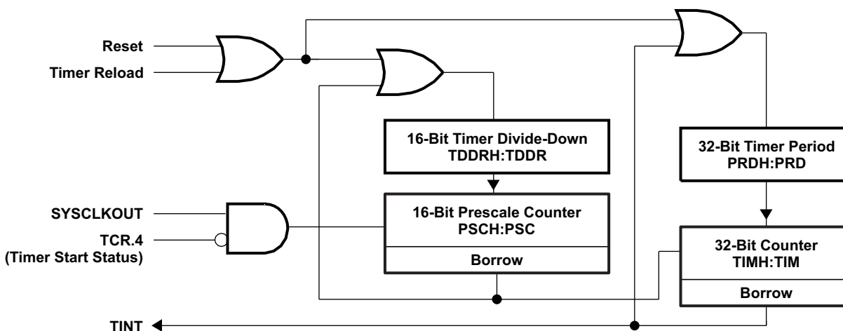
Figure 6-1. CPU-Timers
