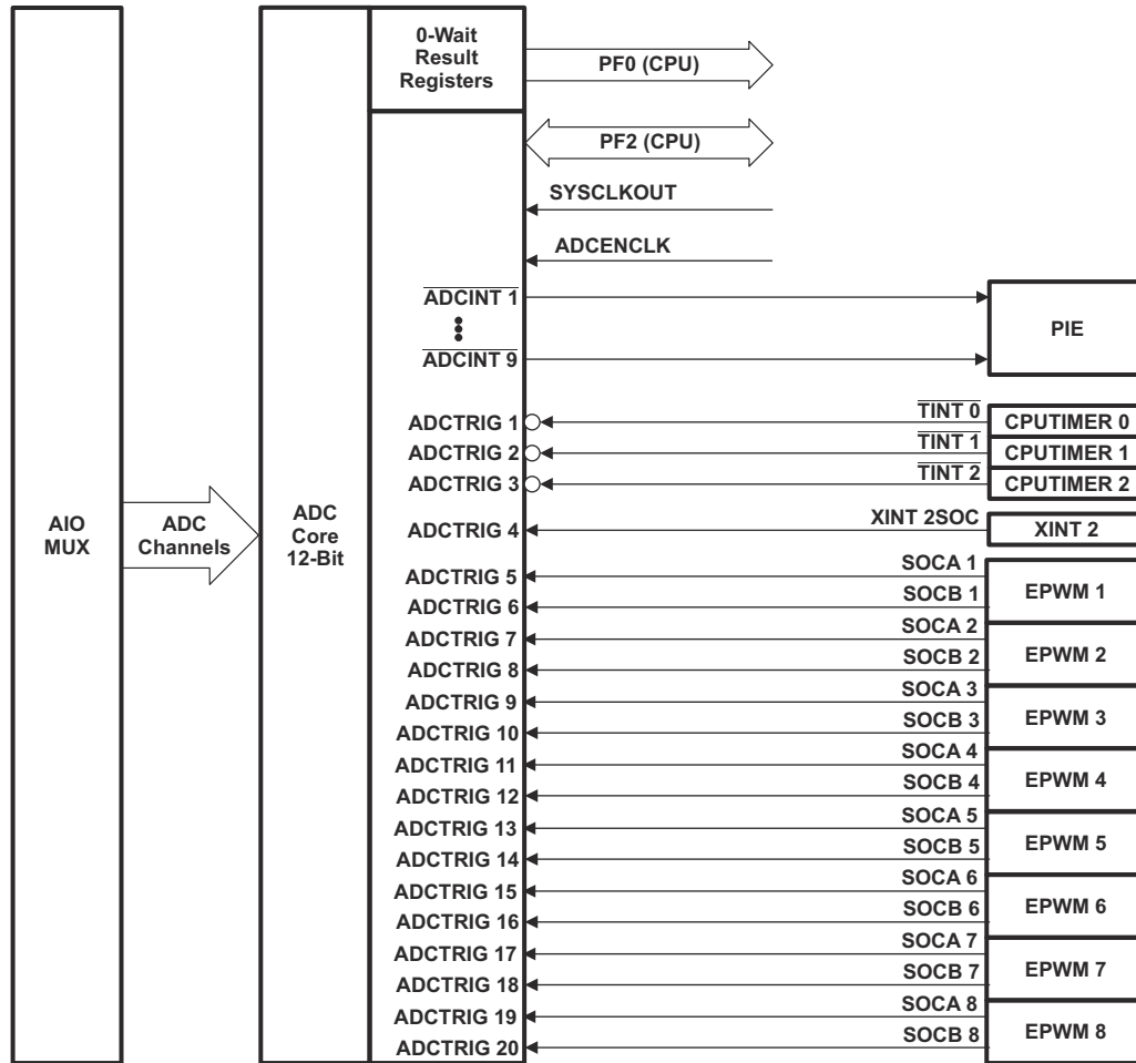
8-21. ADC Connections
