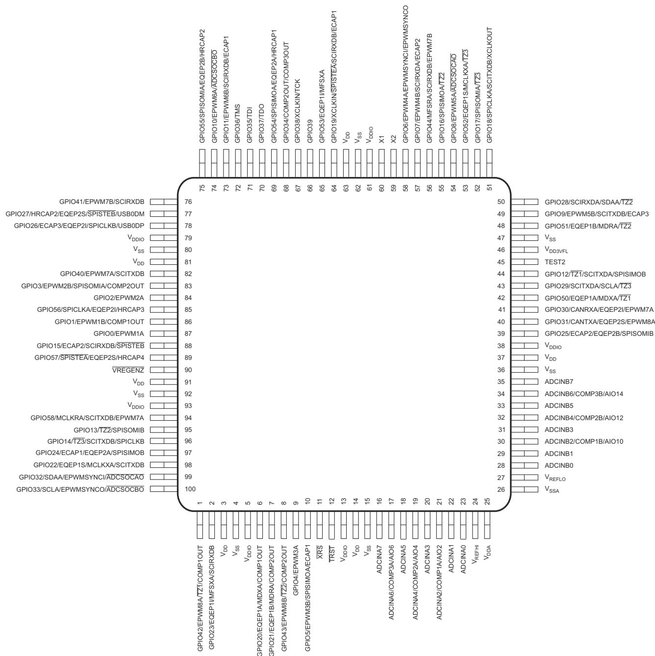
6-2. 100-Pin PZ and PZP Packages (Top View)
