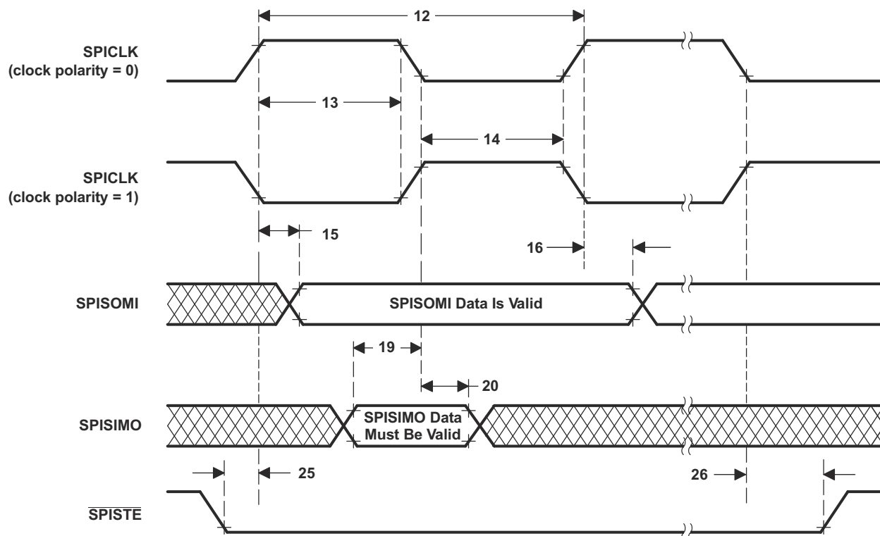
8-35. SPI Slave Mode External Timing (Clock Phase = 0)
