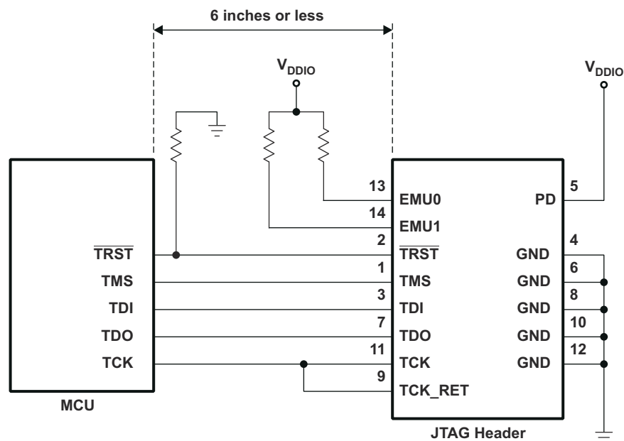
7-3. Debug Probe Connection Without Signal Buffering for the MCU
