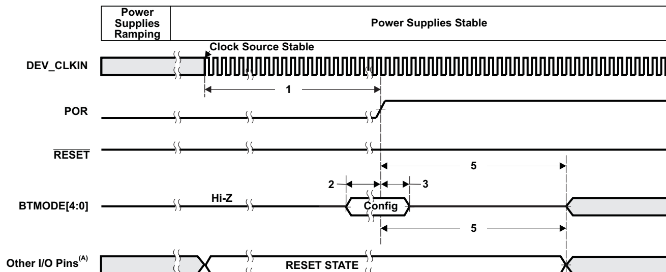
Figure 8-2. Power-Up Timing
