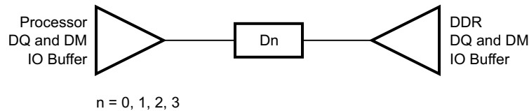
Figure 9-34. DQ/DM Topology
