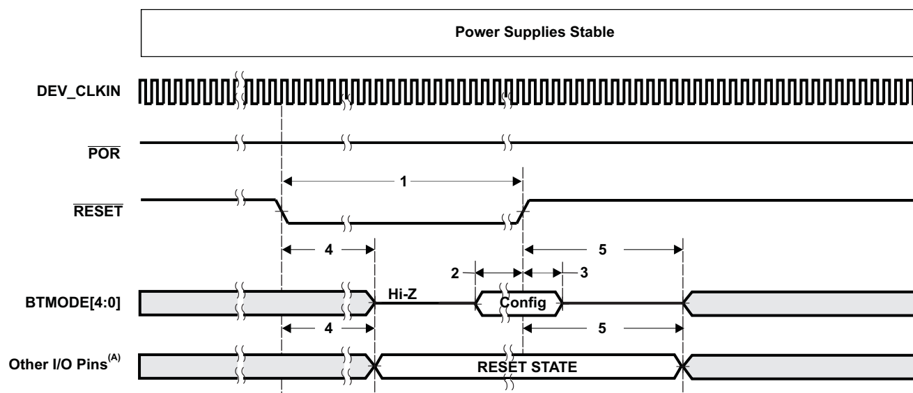
Figure 8-2. Power-Up Timing
