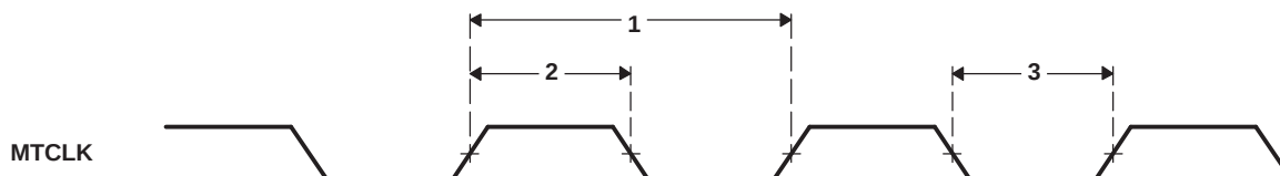
Figure 6-66. MTCLK Timing (EMAC - Transmit)
