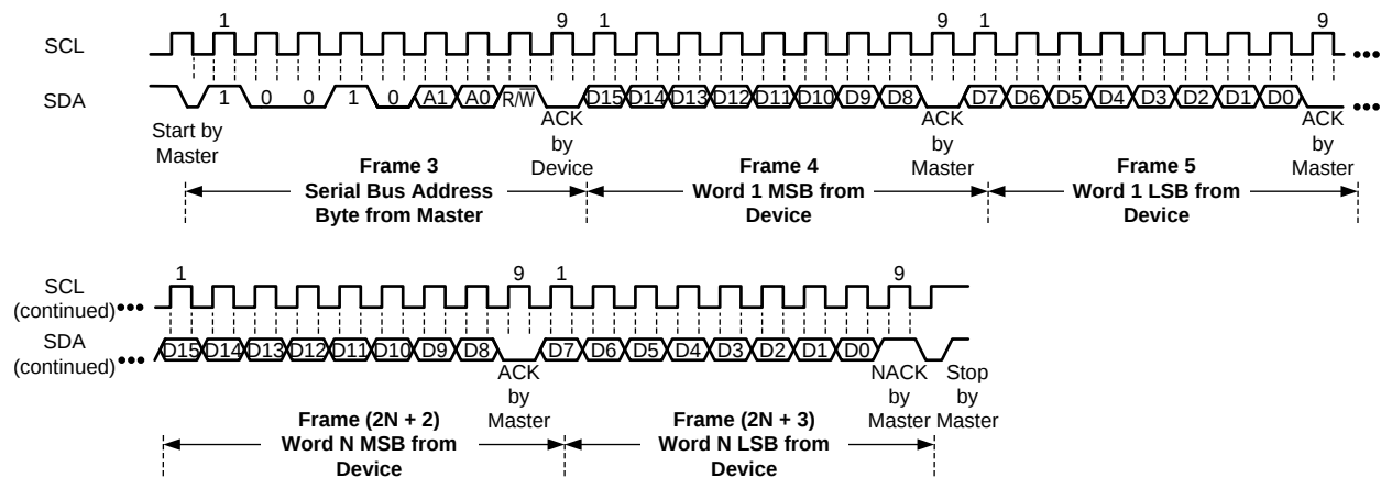
FIG 20. Two-Wire Timing Diagram for Multiple-Word (N-Word) Read Without a Pointer Byte Set
