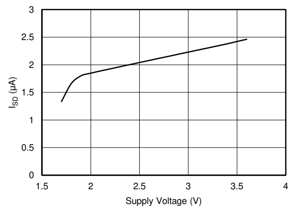
FIG 6-11. Shutdown Quiescent Current vs. Supply Voltage
