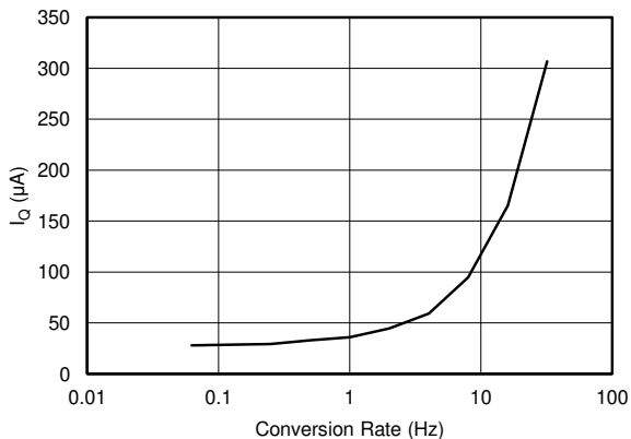
FIG 6-8. Quiescent Current vs. Conversion Rate
