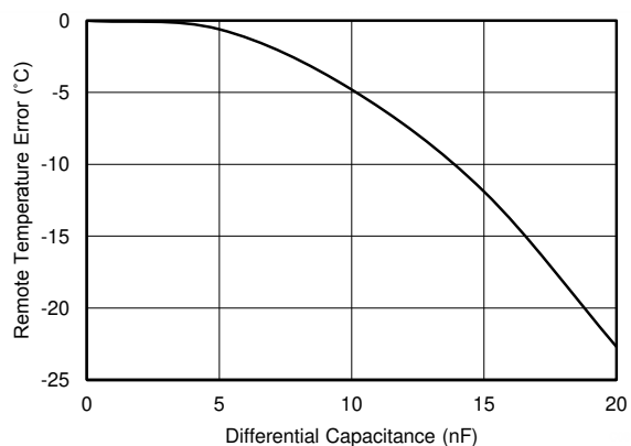
FIG 6-6. Remote Temperature Error vs. Differential Capacitance
