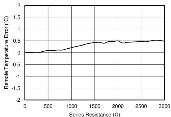
FIG 6-5. Remote Temperature Error vs. Series Resistance
