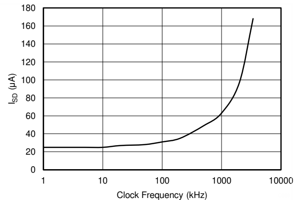
FIG 6-9. Shutdown Quiescent Current vs. SCL Clock Frequency
