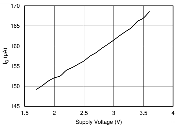
FIG 6-10. Quiescent Current vs. Supply Voltage (At Default Conversion Rate of 16 Conversions per Second)
