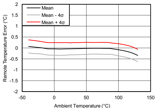
FIG 6-3. Remote Temperature Error vs. Temperature
