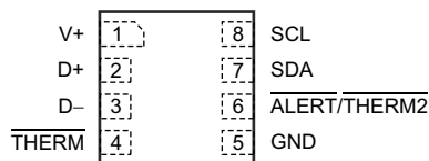
图 5-1. DQF Package 8-Pin WSON Top View
