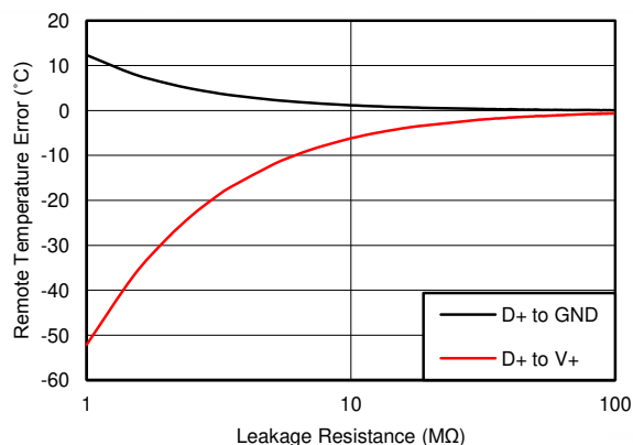
FIG 6-4. Remote Temperature Error vs. Leakage Resistance
