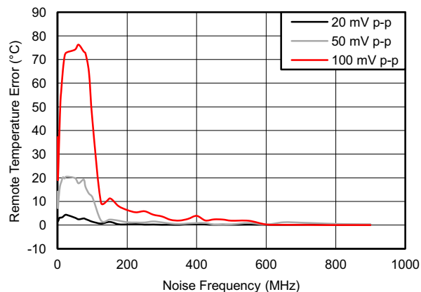
FIG 6-7. Remote Temperature Error vs. Remote Channel Noise Frequency
