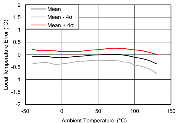
FIG 6-2. Local Temperature Error vs. Temperature
