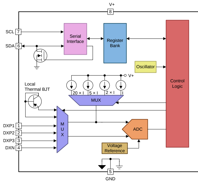
Figure 14. The TMP423-Q1 With Three Remote Diode Inputs
