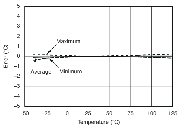
FIG 7-6. 10°C Hysteresis Error vs Temperature
