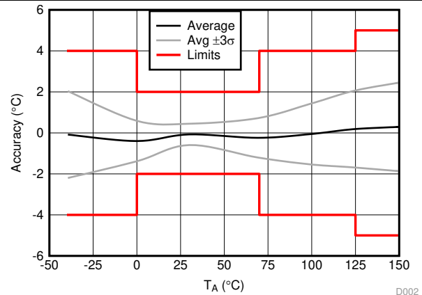
FIG 2. Accuracy vs. T_A Temperature (A4 Accuracy Level)
