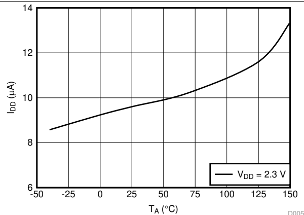
FIG 5. Supply Current vs. Temperature
