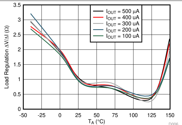
FIG 4. Changes in Accuracy vs. Ambient Temperature (Due to Load)
