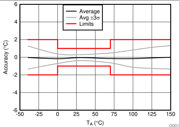
FIG 1. Accuracy vs. T_A Temperature (A2 Accuracy Level)
