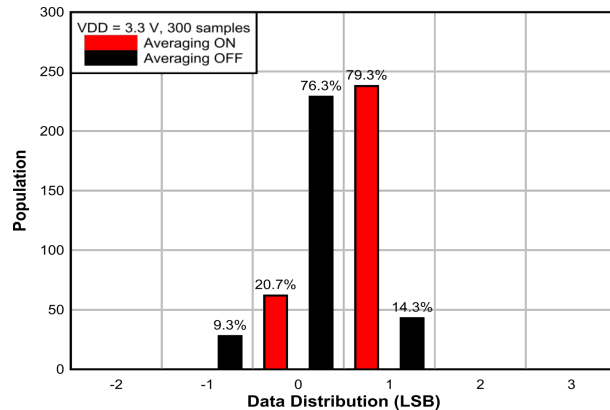
7-4. Temperature Measurement Noise Distribution at -55°C
