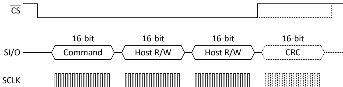
✎ 8-9. TMP126 Communication Overview
