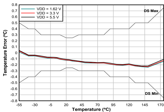
Figure 9-2. Average Temperature Accuracy
