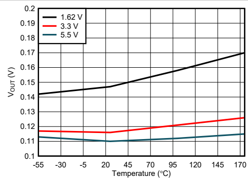
7-9. ALERT Output vs. Temperature
