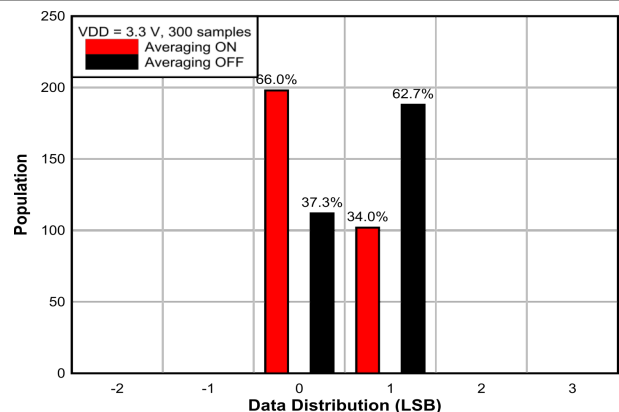
7-3. Temperature Measurement Noise Distribution at 25°C
