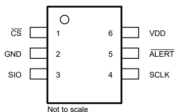
図 6-1. DCK 6-pin SC70 Top View
