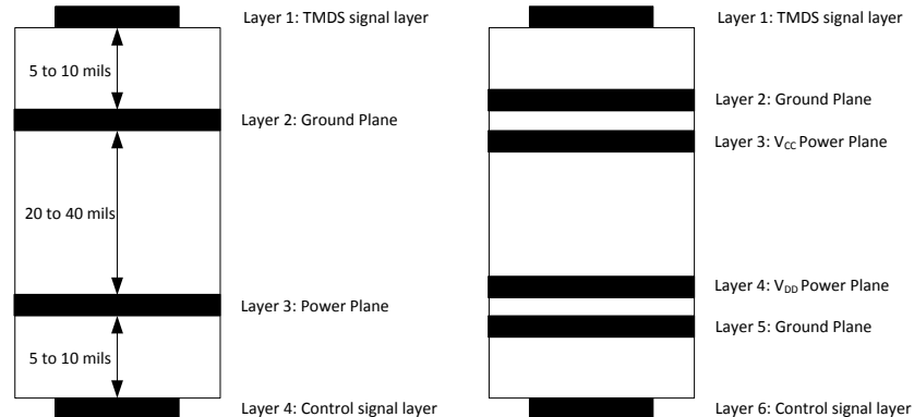
Figure 62. Recommended 4 or 6 Layer PCB Stack
