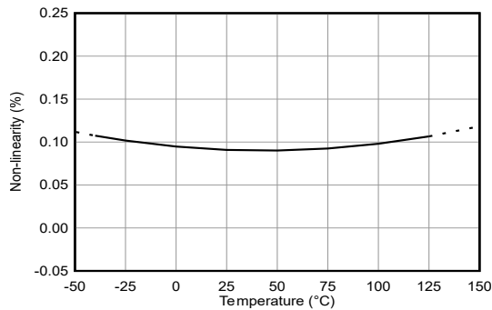
6-5. Non-Linearity vs Temperature
