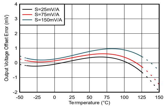
6-2. Offset Error vs Temperature: TMCS1133Axx-Q1 Device Options
