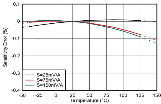
6-1. Sensitivity Error vs Temperature
