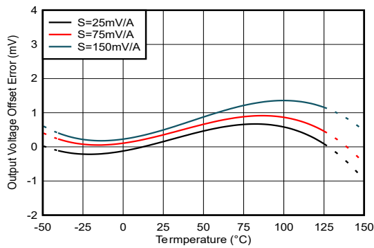
6-3. Offset Error vs Temperature: TMCS1133Bxx-Q1 Device Options
