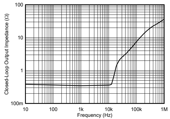
6-10. Output Impedance vs Frequency
