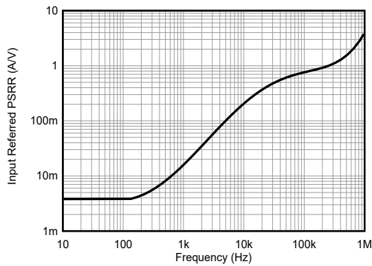
6-9. PSRR vs Frequency
