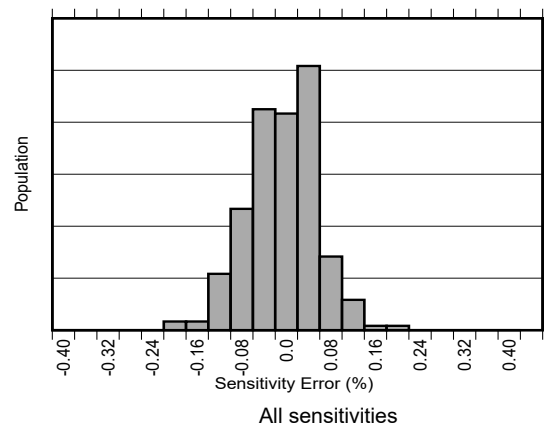
6-6. Sensitivity Error Production Distribution
