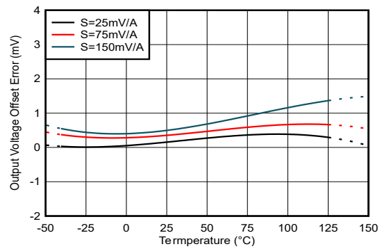
6-4. Offset Error vs Temperature: TMCS1133Cxx-Q1 Device Options
