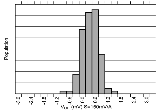
Figure 6-10. Offset Error Production Distribution
