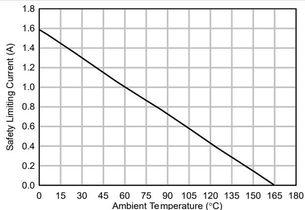
Figure 6-24. Thermal Derating Curve for Safety-Limiting Current, Side 2
