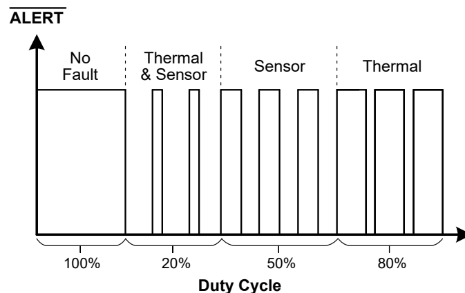
Figure 8-9. Sensor Diagnostics Waveform
