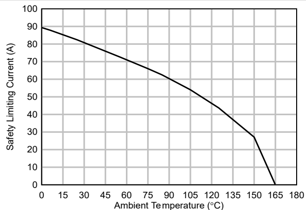
Figure 6-23. Thermal Derating Curve for Safety-Limiting Current, Side 1
