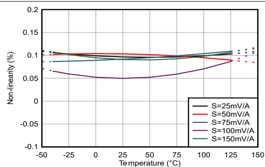
Figure 6-4. Non-Linearity vs Temperature
