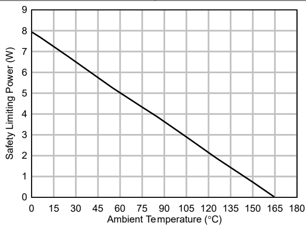
Figure 6-25. Thermal Derating Curve for Safety-Limiting Power
