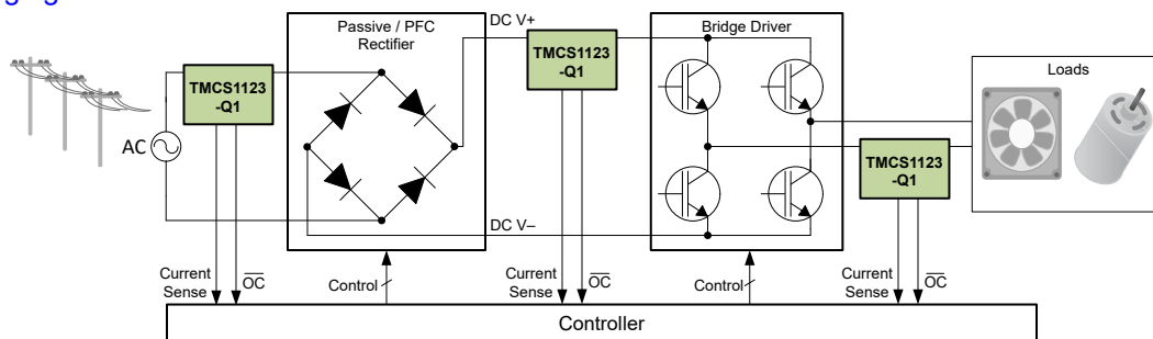
Typical Application
