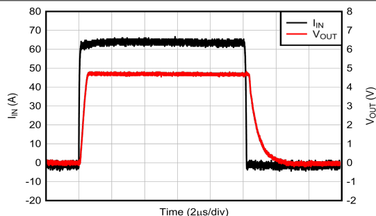
Figure 6-17. Current Overload Response
