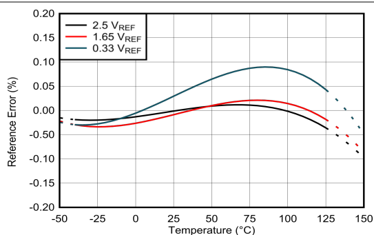
Figure 6-3. Reference Error vs Temperature
