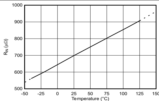
Figure 6-22. Input Conductor Resistance vs Temperature
