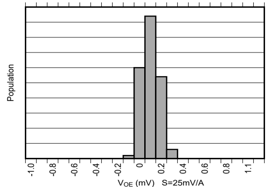
Figure 6-6. Offset Error Production Distribution
