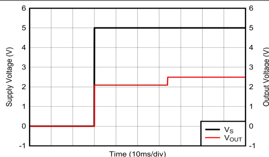
Figure 6-18. Startup Transient Response
