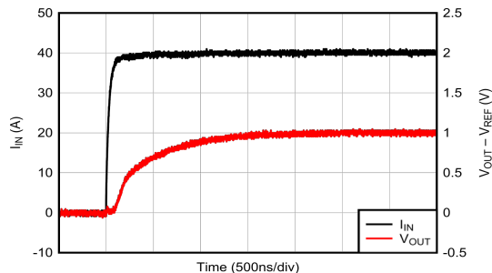
Figure 6-15. Voltage Output Step Response, Rising
