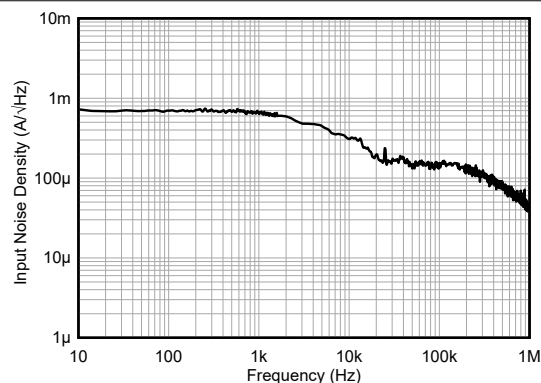
Figure 6-21. Input-Referred Noise Density vs Frequency
