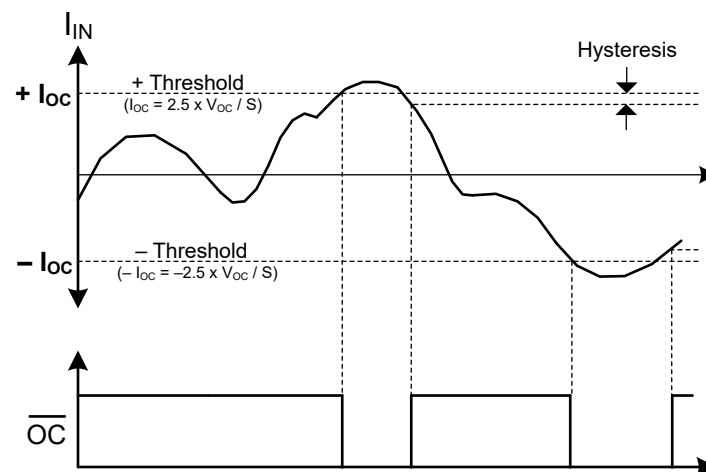
8-8. Overcurrent Output Response
