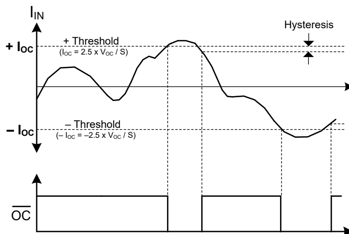
図 8-8. Overcurrent Output Response
