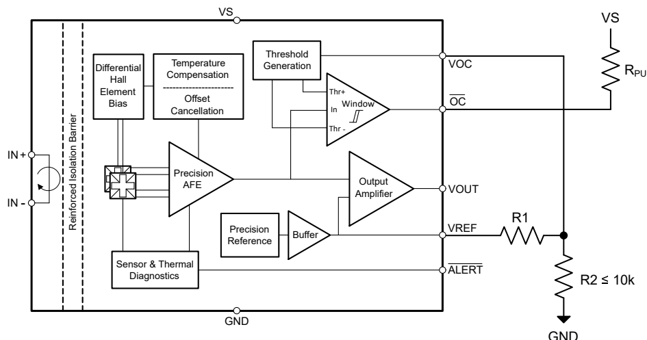
図 8-7. User Configurable Overcurrent Threshold Using Zero Current Output Reference Voltage
