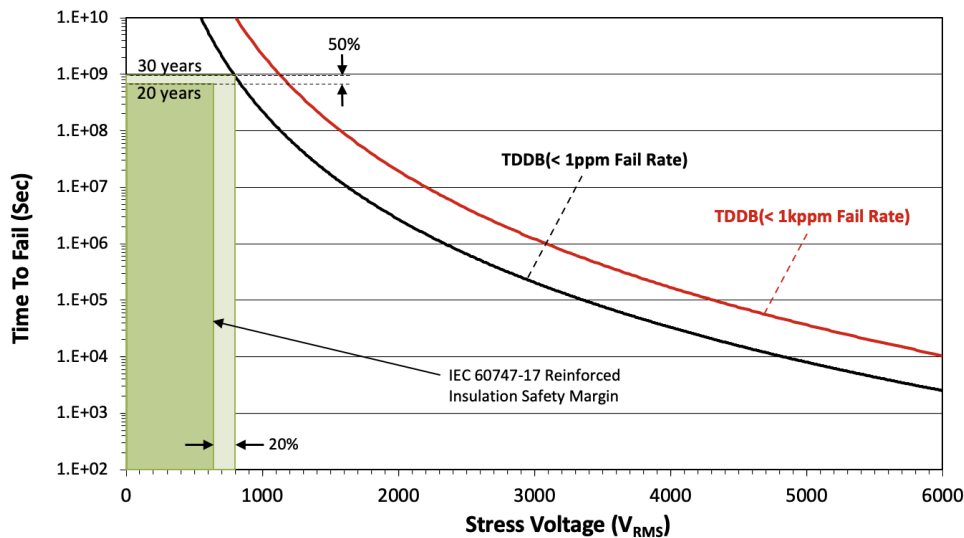
8-2. Insulation Lifetime
