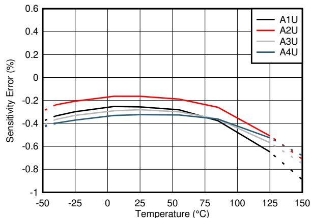
FIG 7-2. TMCS1101AxU Sensitivity Error vs Temperature
