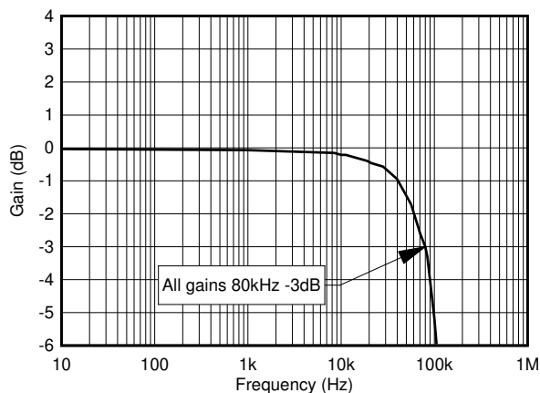
FIG 9-9. Normalized Gain, All Variants
