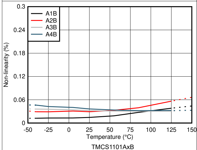
FIG 7-5. Non-Linearity vs. Temperature
