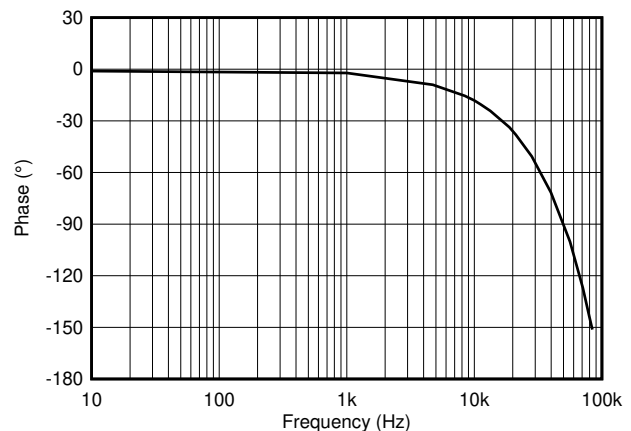
FIG 9-10. Normalized Phase, All Variants
