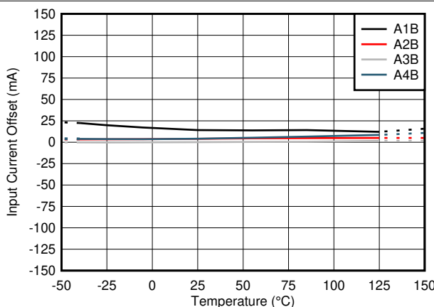
FIG 7-3. TMCS1101AxB Input Offset Current vs Temperature
