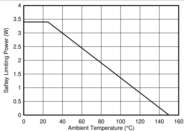
図 7-30. Thermal Derating Curve for Safety-Limiting Power
