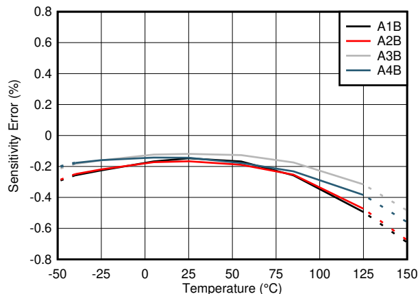
FIG 7-1. TMCS1101AxB Sensitivity Error vs Temperature
