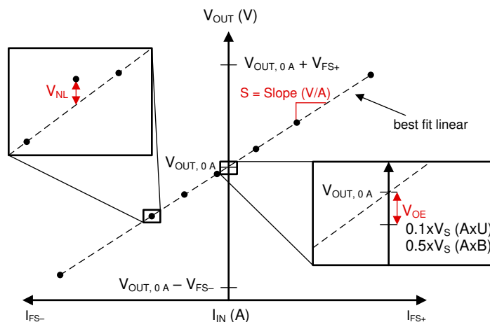
図 8-1. Sensitivity, Offset, and Nonlinearity Error
