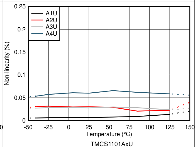
FIG 7-6. Non-Linearity vs. Temperature
