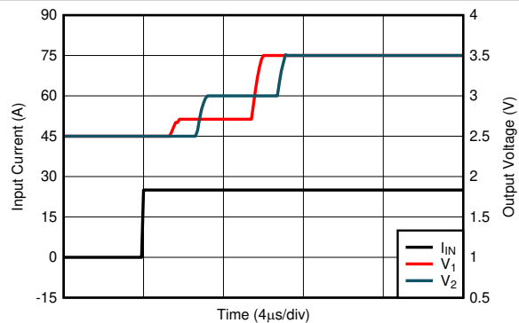
7-23. Voltage Output Step, Rising
