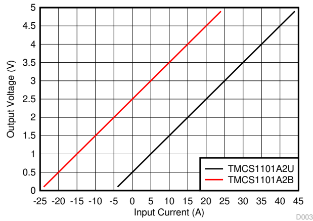
図 9-14. Output Voltage Relationship to Input Current for TMCS1101A2B and TMCS1101A2U
