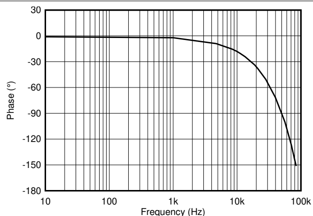
7-18. Phase vs. Frequency, All Gains
