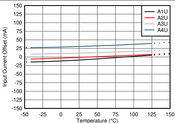
FIG 7-4. TMCS1101AxU Input Offset Current vs Temperature
