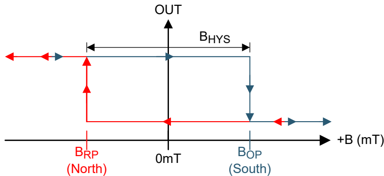
図 7-3. Bipolar Latch Active Low Functionality
